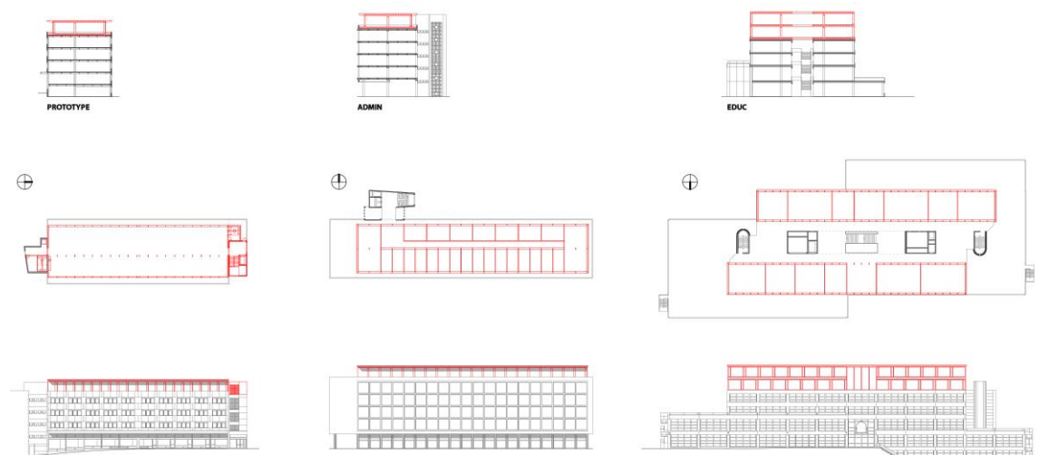
Figure 1. Different building configurations studied during the system's development to check its adaptability to various dimensions of pre-existing structural grids, façade designs and orientations. Elements in red refer to the new construction, while elements in black refer to the existing building.
