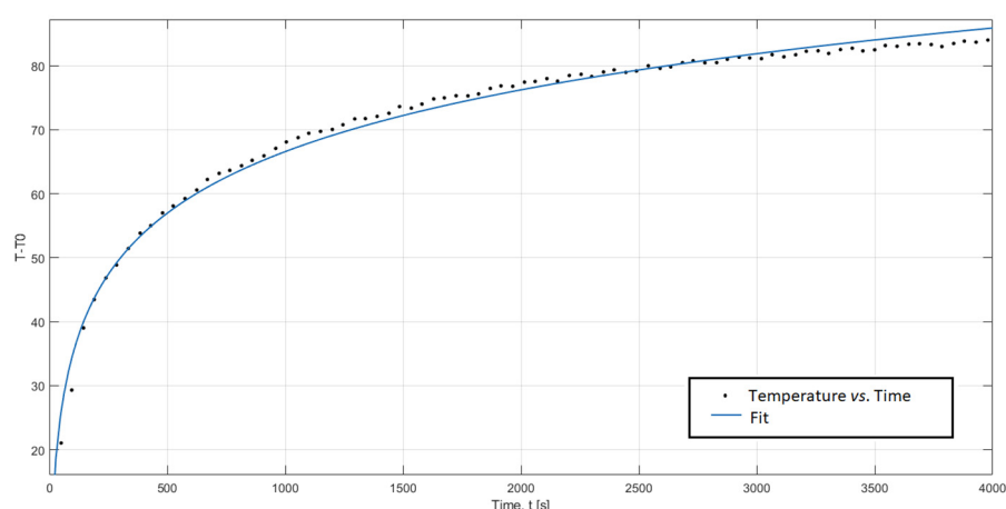
Figure 8. Fit for the Skamol SM-65 sample.
