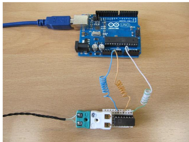
Figure 4. Datalogger.
