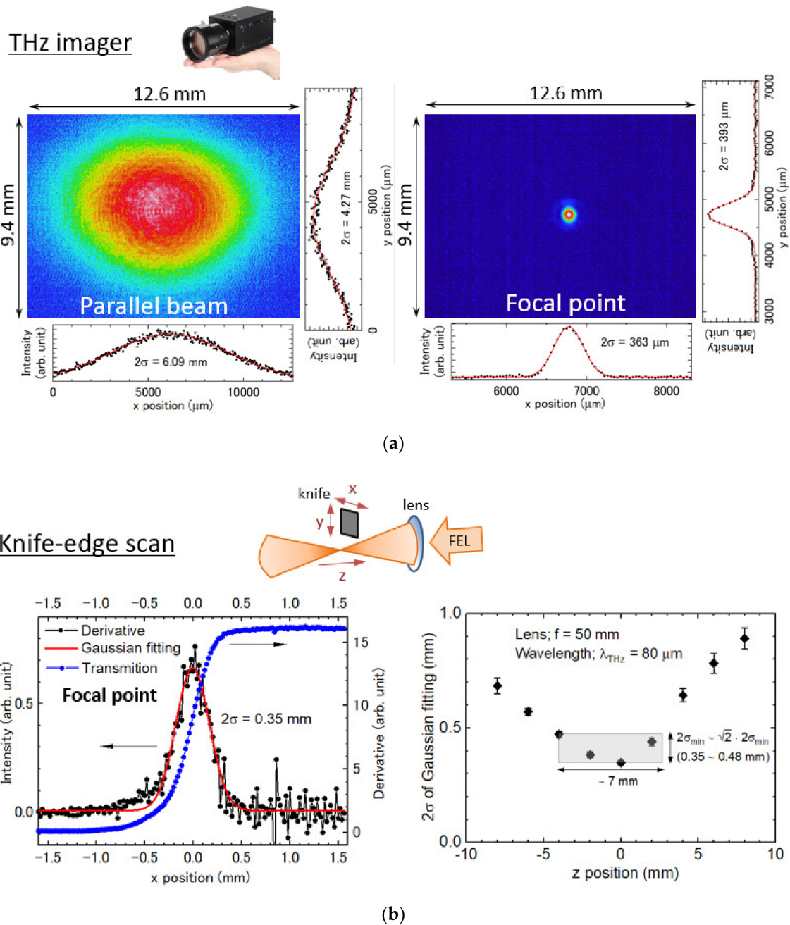
Figure 4. The beam profiles of the ISIR FEL (a) taken with a THz camera for the parallel beam (left) and at the focal point (right), and (b) the spatial resolution measured with the knife-edge scan around the focal point.
