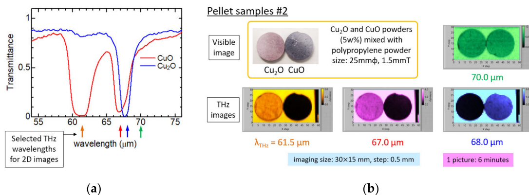
Figure 6. (a) Comparison of transmittance spectra of \text{Cu}_2\text{O} and CuO by in situ observation; (b) 2D images of \text{Cu}_2\text{O} and CuO pellets collected in transmission at several THz wavelengths.
