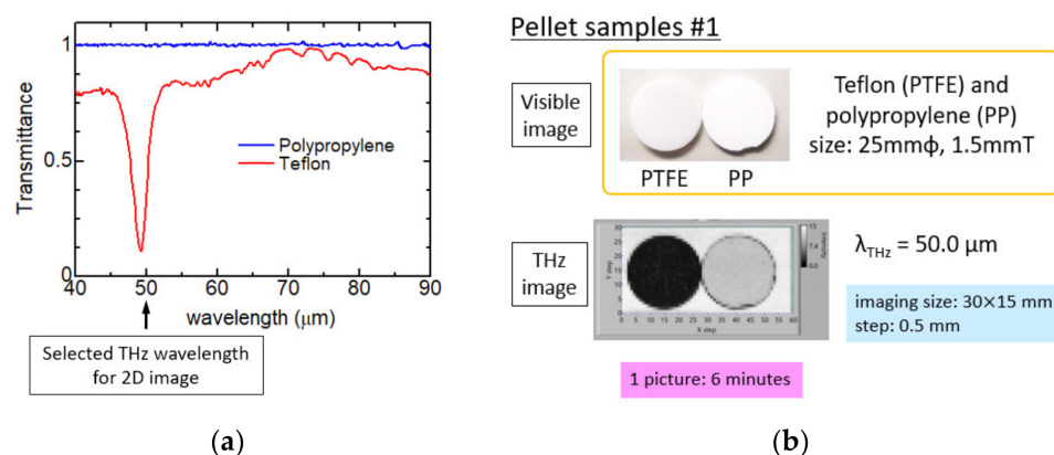
Figure 5. (a) Comparison of transmittance spectra of polytetrafluoroethylene (PTFE) and polypropylene (PP) by in situ observation; (b) 2D images of PTFE and PP pellets collected in transmission at \lambda_{\text{THz}} = 50\text{ }\mu\text{m} .
