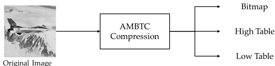
Figure 1. Flow of AMBTC compression phase.
