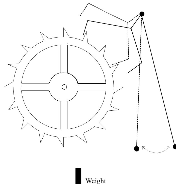
Figure 1. Simplified diagram of an escapement mechanism.
