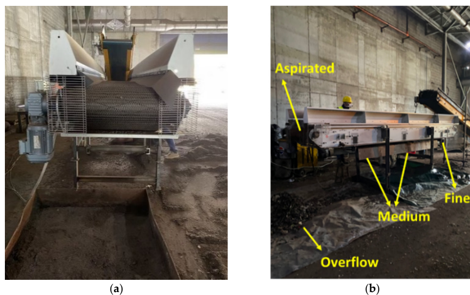
Figure 4. Final conveyor belt (a) and products obtained during the test (b).
