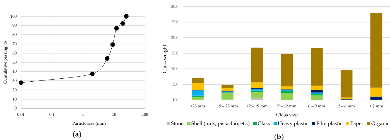
Figure 6. Granulometric curve of the initial sample of overflow (a); composition in weight of each class size (b).
