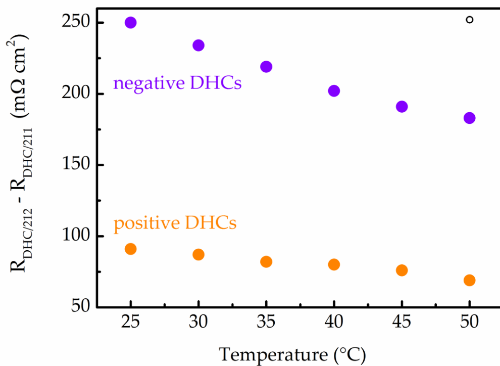
Figure S1. Difference in resistance of positive and negative DHCs using NR-211 and NR-212 membranes at different temperatures.
