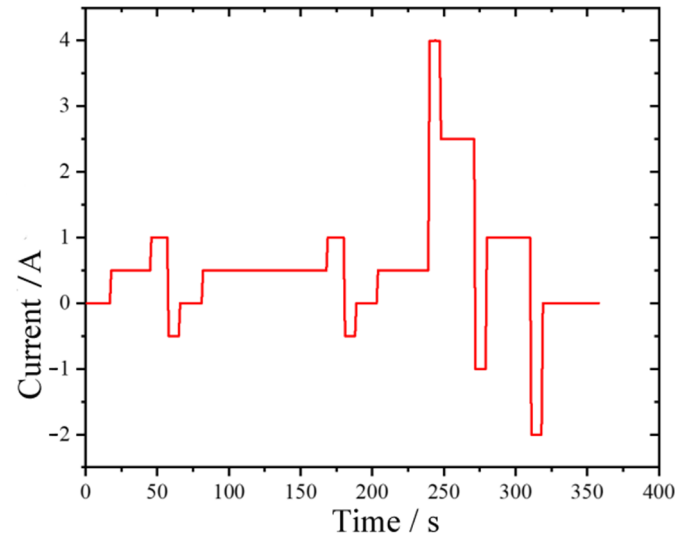
Figure 2. Current profile of a single DST cycle.
