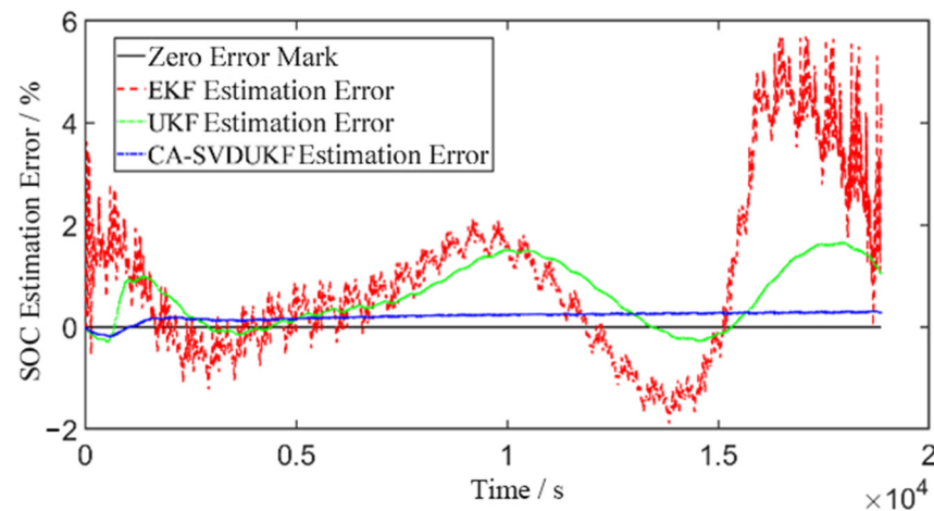
Figure 12. SOC estimation errors of the battery under the US06 condition.
