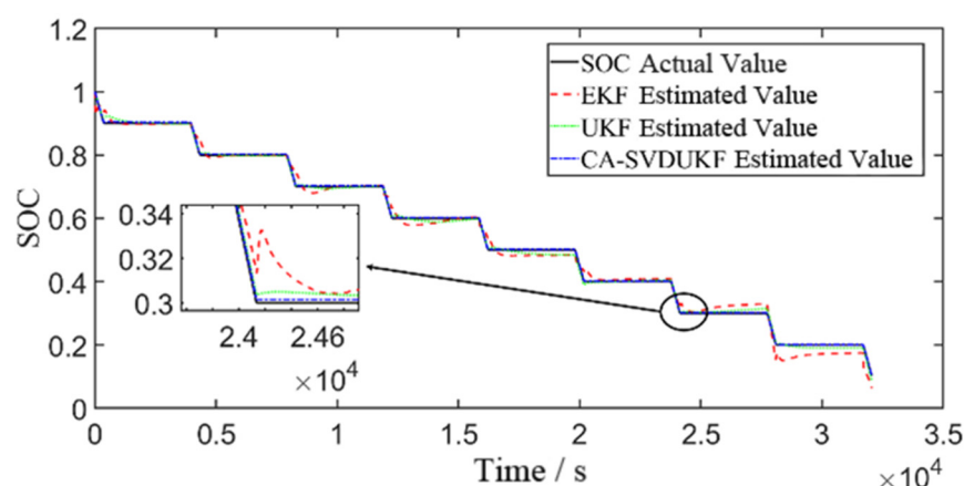
Figure 6. SOC estimation results of the battery under the constant pulse condition.
