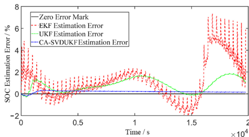
Figure 9. SOC estimation errors of the battery under the DST condition.
