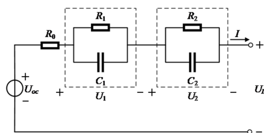
Figure 1. Second-order RC equivalent circuit model.
