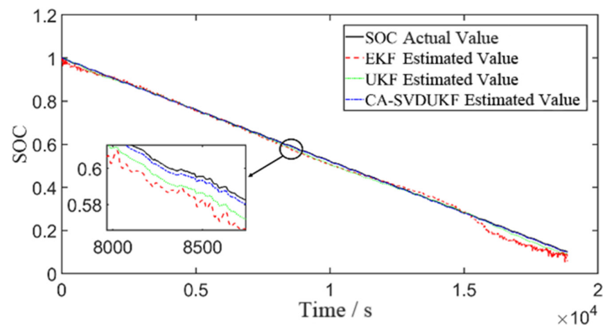
Figure 11. SOC estimation results of the battery under the US06 condition.
