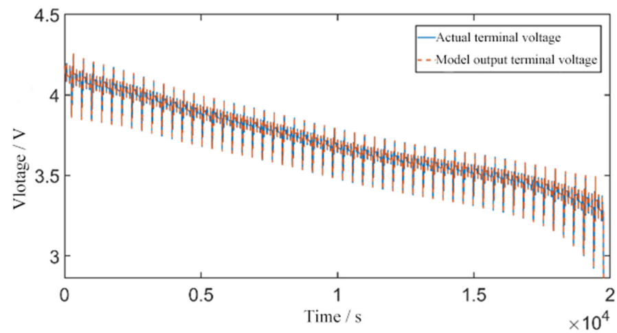
Figure 3. Comparison of terminal voltage under DST profile with online identification.
