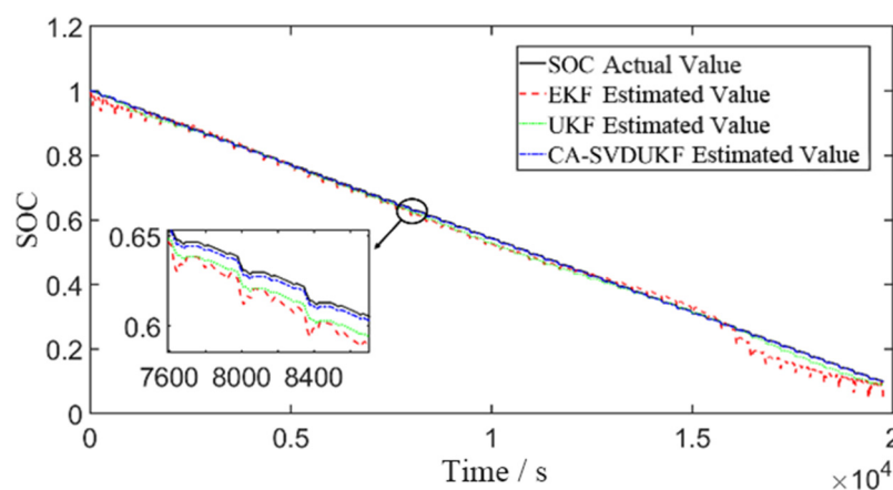
Figure 8. SOC estimation results of the battery under the DST condition.
