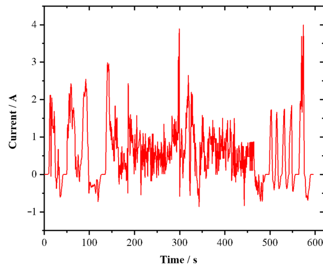
Figure 10. Single-cycle current profile under the US06 condition.
