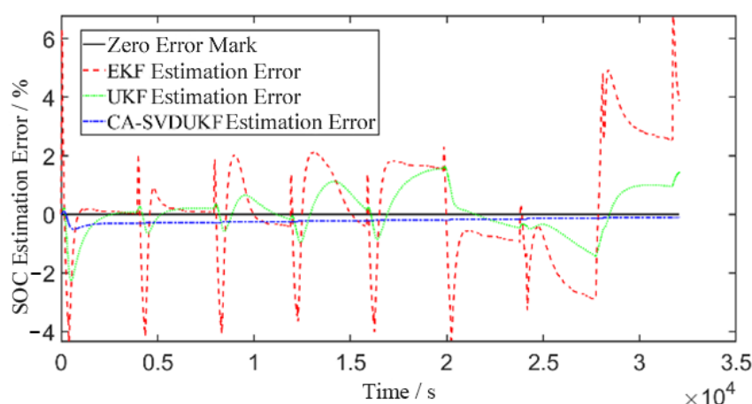
Figure 7. SOC estimation errors of the battery under the constant pulse condition.
