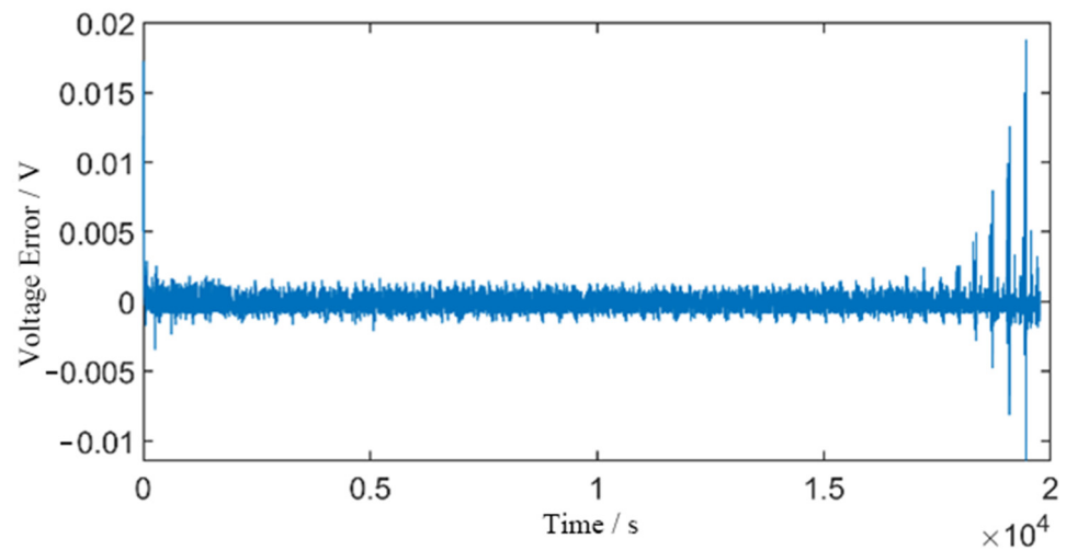
Figure 4. Terminal voltage error under DST profile with online identification.
