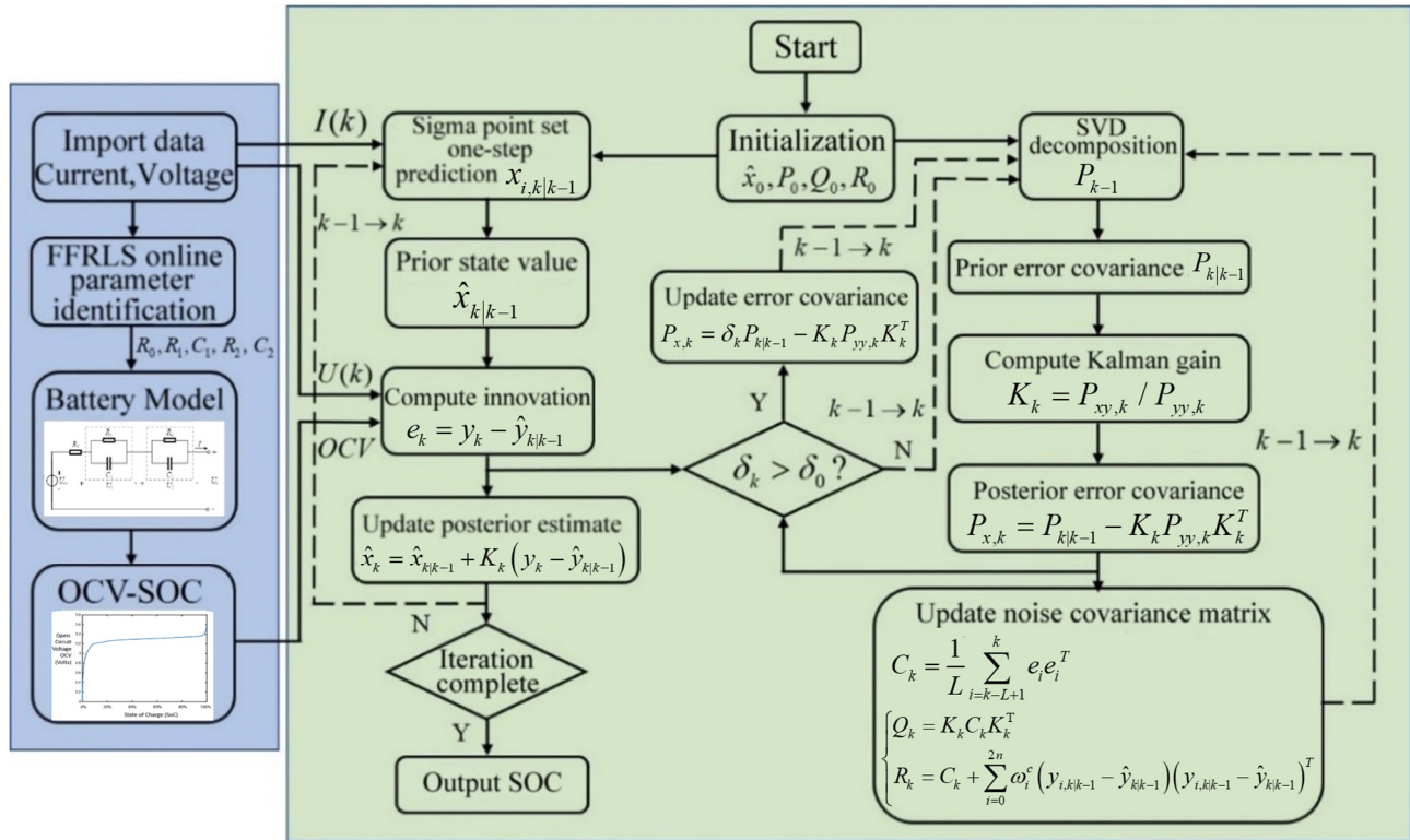
Figure 5. Flowchart of the CA-SVDFKF algorithm.
