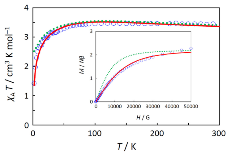
Figure S1. The \chi T versus T plot and the M versus H plot (insertion). The observed data ( \circ ) and the theoretical curves ( - ) with considering \theta and ( \cdots ) without considering \theta .
