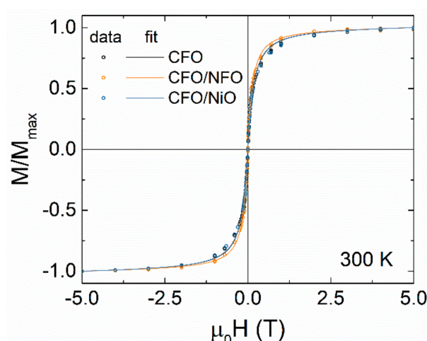
Figure 6. Measured and fitted with the Langevin–Chantrell method M–H cycles at 300 K.
