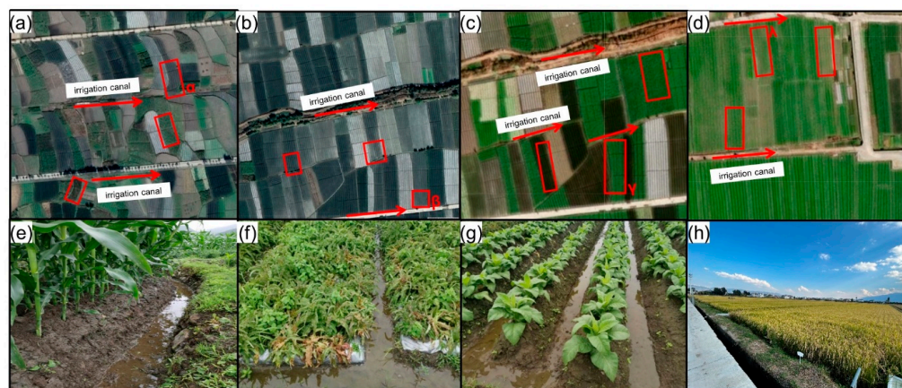
Figure 2. Distribution of long-term observation sites of baseflow in (a–d) surrounding soil profiles of sites 1, 2, 3 and 4 in Figure S1, respectively. Field photos of (e–h) of “α”, “β”, “γ” and “λ” in (a–d), respectively. The red rectangles represent the long-term observation fields of baseflow, and the red arrows are the irrigation canals.
