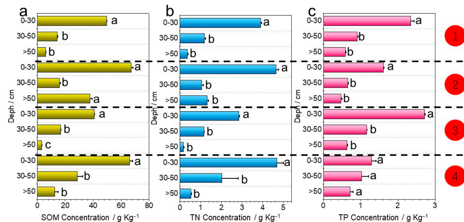
Figure 4. Soil nutrient concentrations of (a) SOM; (b) TN; and (c) TP in different soil depths. Profiles 1–4 are distributed from Mount Cangshan to Lake Erhai, with crops of corn, vegetable, tobacco and rice, respectively. Significant differences are noted using “a–c”.
