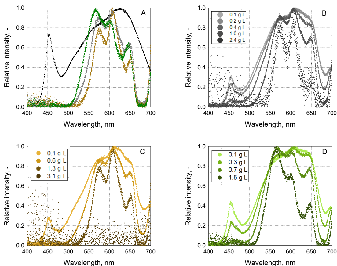
Figure 5. Light spectra measurements on the light-adverted side of the flat-plate gas-lift photobioreactor at different process times and biomass concentrations. The light measurements were always taken at the same location in the reactor (in the middle of the reactor). (A) Comparison of the measured spectra of I. galbana (brown) in monoculture, N. oceanica (green) in monoculture, and a co-culture of I. galbana and N. oceanica (grey) at an average biomass concentration of 1.1 \pm 0.2 \text{ g L}^{-1} and an incident PPFD of 2000 \mu\text{mol m}^{-2} \text{ s}^{-1} . (B) Spectra of the co-culture of I. galbana and N. oceanica at different biomass concentrations and the same incident PPFD of 2000 \mu\text{mol m}^{-2} \text{ s}^{-1} . (C) Spectra of the monoculture of I. galbana at different biomass concentrations and the same incident PPFD of 2000 \mu\text{mol m}^{-2} \text{ s}^{-1} . (D) Spectra of the monoculture of N. oceanica at different biomass concentrations and the same incident PPFD of 2000 \mu\text{mol m}^{-2} \text{ s}^{-1} .
