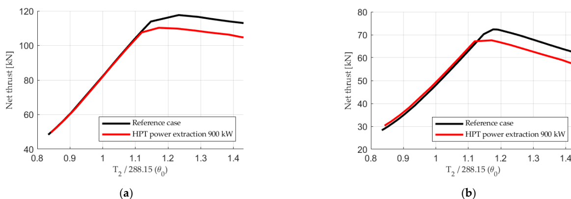
Figure 11. Net thrust plotted versus \theta_0 ( T_2/288.15 ); (a) Maximum augmented power; (b) Maximum non-augmented power.
