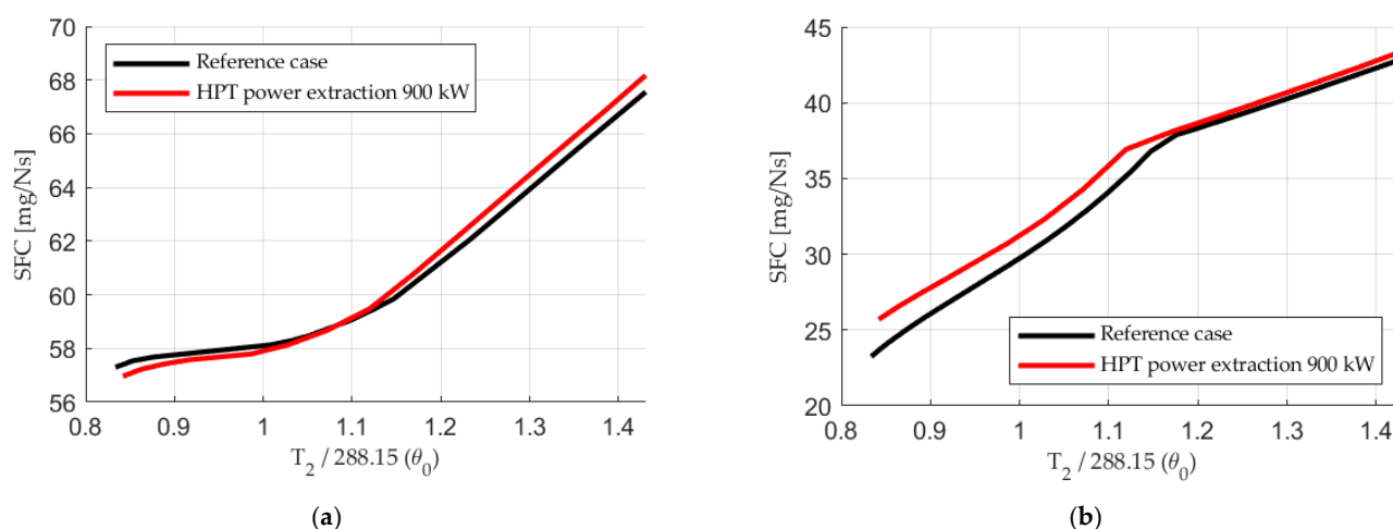
Figure 12. SFC plotted versus \theta_0 ( T_2/288.15 ); (a) Maximum augmented power; (b) Maximum non-augmented power.
