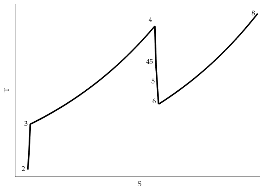
Figure 2. Schematic T-S diagram. Use of afterburner illustrated.
