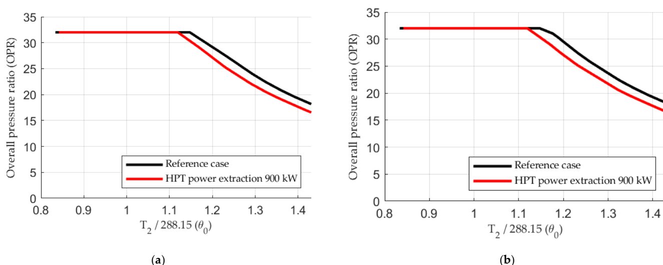
Figure 10. OPR plotted versus \theta_0 ( T_2/288.15 ); (a) Maximum augmented power; (b) Maximum non-augmented power.
