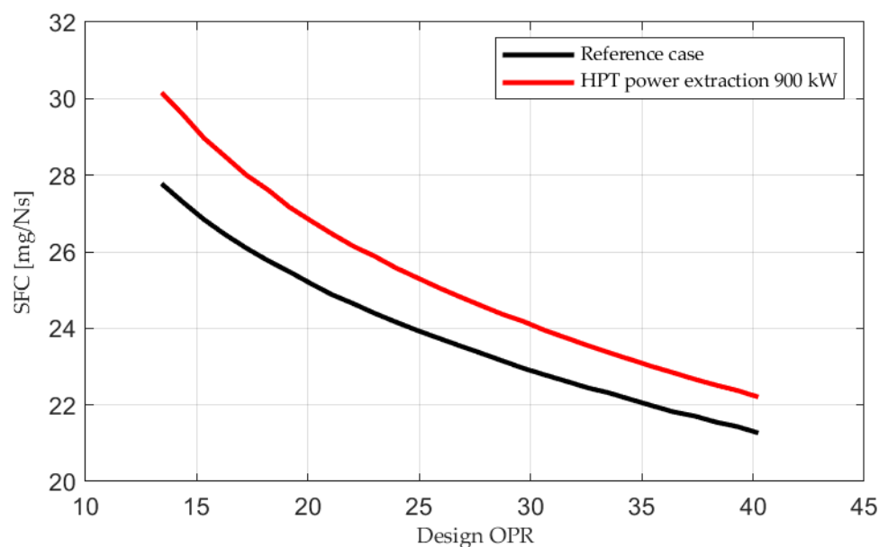
Figure 13. Point 1 of the mission. SFC plotted versus design point OPR.
