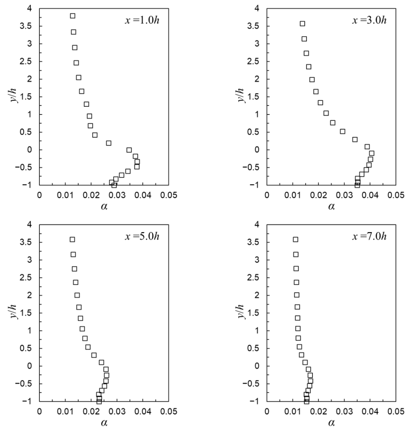
Figure 9. Computational results of mean void fraction distributions at different streamwise sections at Re = 64,800 , \sigma = 0.328 , and initial \alpha = 1\% for ER = 1.07 channel.
