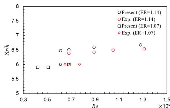
Figure 5. Variation of reattachment length with Reynolds number and expansion ratio.
