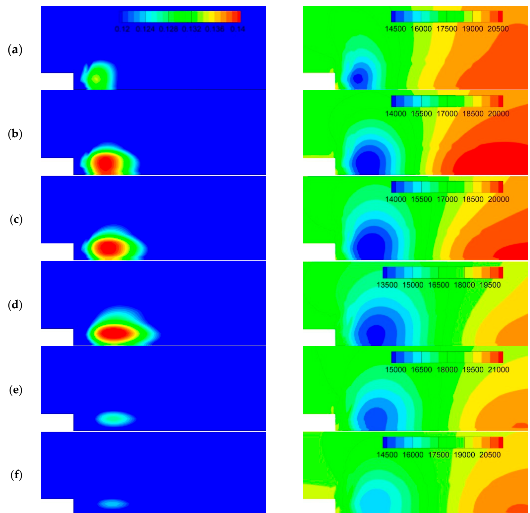
Figure 10. Time evolution of void fraction (left) and pressure (right) distribution at Re = 31,000 , \sigma = 1.420 , and initial \alpha = 10\% for ER = 1.07 channel. (a) T_0 ms. (b) T_0 + 30 ms. (c) T_0 + 60 ms. (d) T_0 + 160 ms. (e) T_0 + 220 ms. (f) T_0 + 260 ms.
