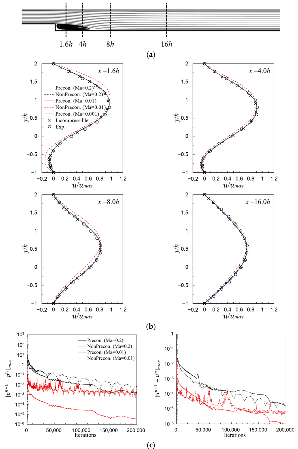
Figure 3. Computational results of a backward-facing step channel for gas phase flow at Re = 100 , and ER = 1.5 : (a) Streamline and cross-sections for measurement; (b) Streamwise velocity profiles at several Mach numbers; (c) Convergence histories.
