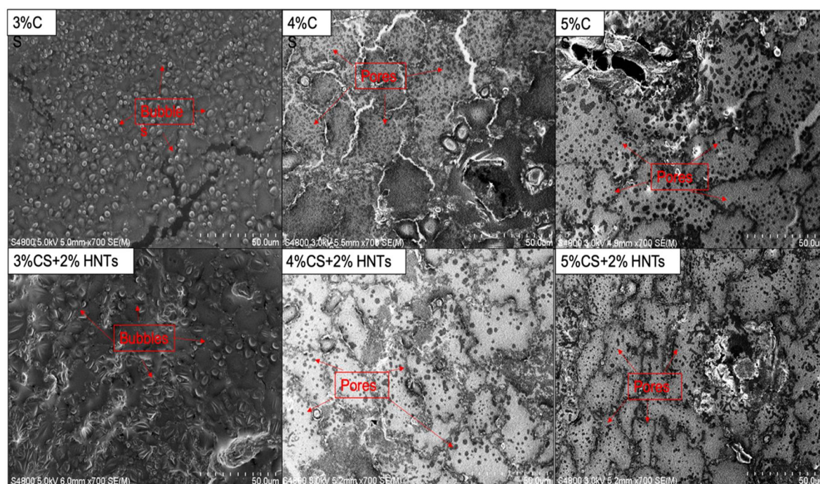
Figure 10. SEM images of cross-section for different hydrogel composites. The arrows in the picture of 3% chitosan (3%C) and its HNTs composites (3%CS + 2%HNTs) point to the example of bubbles. The arrows in the picture of 4% chitosan (4%C) and 5% chitosan (5%C) and their hydrogel composites (4%CS + 2%HNTs and 5%CS + 2%HNTs) point to the example of pores.
