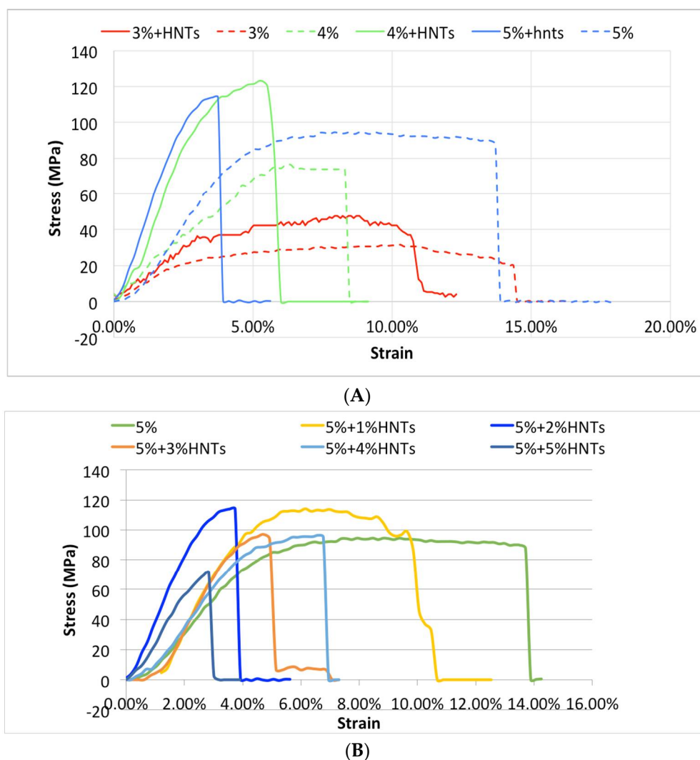
Figure 3. The stress-strain profile of CS and CS/HNTs. (A) Tensile test of pure chitosan (CS) with the HNT additive groups (CS/HNTs). In this graph, every CS/HNT compound has a higher stress value compare to CS group. (3% CS/2% HNTs > 3% CS, 4% CS/2% HNTs > 4% CS, 5% CS/2% HNTs > 5% CS). Simultaneously, a higher concentration of chitosan showed higher stress values (5% > 4% > 3%), however, the strain values displayed a different response (5% < 4% < 3%). (B) 5% CS/1% HNTs showed a major improvement in elongation, while 5% CS/2% HNTs showed the greatest improvement in strength. Increasing of number of HNTs gradually decreased its reinforcement ability, until at these concentrations (CS/HNTs (5% CS/ 5% HNTs), the nanocomposites was weaker and more fragile than pure CS. The step-wise failure behavior (slippage) at the end of each profile represents the fracture point of each specimen.
