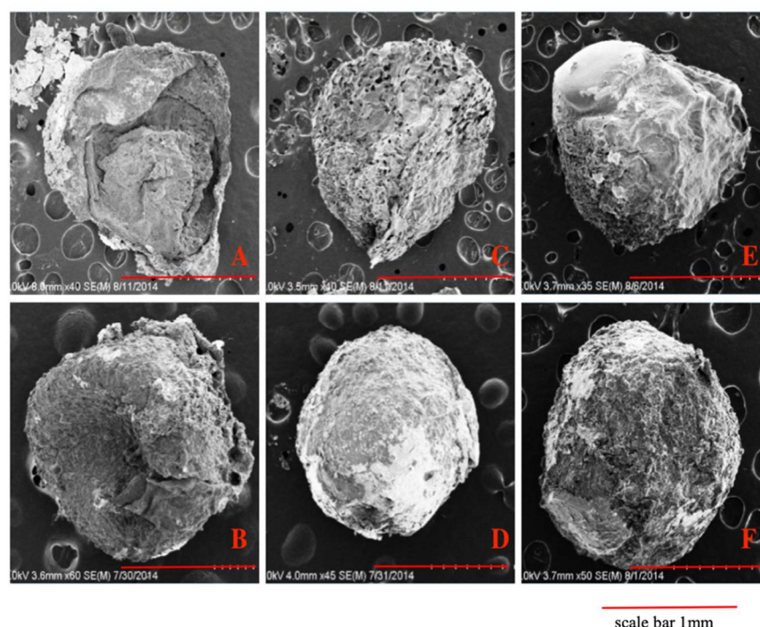
Figure 1. SEM images of pure chitosan hydrogel beads with increased chitosan concentration (A, C, E) and chitosan/ Halloysite nanotubes (HNTs) wt./wt. composites (B, D, F). (A) 3% chitosan (CS), (B) 3% CS/2% HNTs, (C) 4% CS, (D) 4% CS/2% HNTs, (E) 5% CS, (F) 5% CS/ 2% HNTs.
