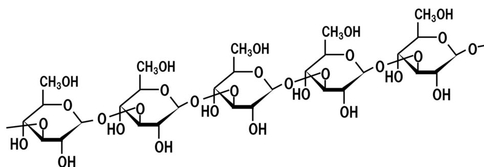
Figure 13. Chemical structure of beta-glucan.
