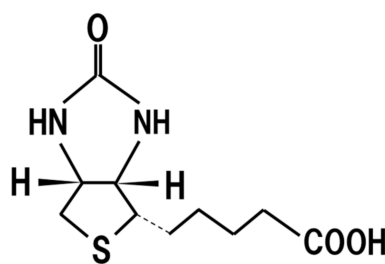
Figure 12. Chemical structure of biotin.
