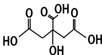
Figure 14. Chemical structure of citric acid.
