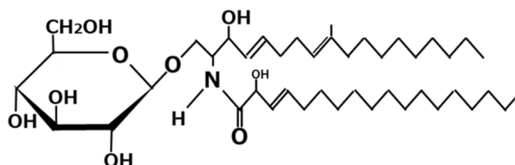
Figure 2. Chemical structure of glycosylceramide.
