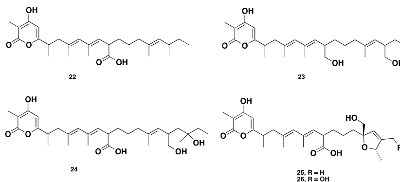
Figure 3. Chemical structures of 22–26.
