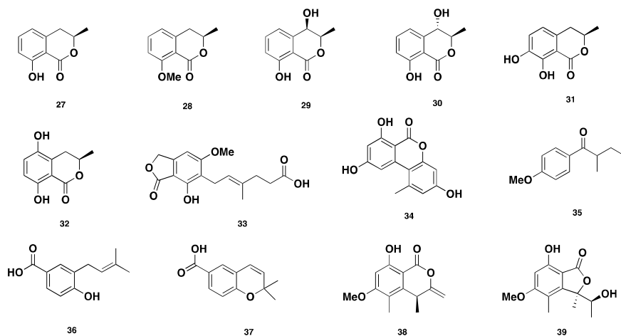
Figure 4. Chemical structures of 27–39.
