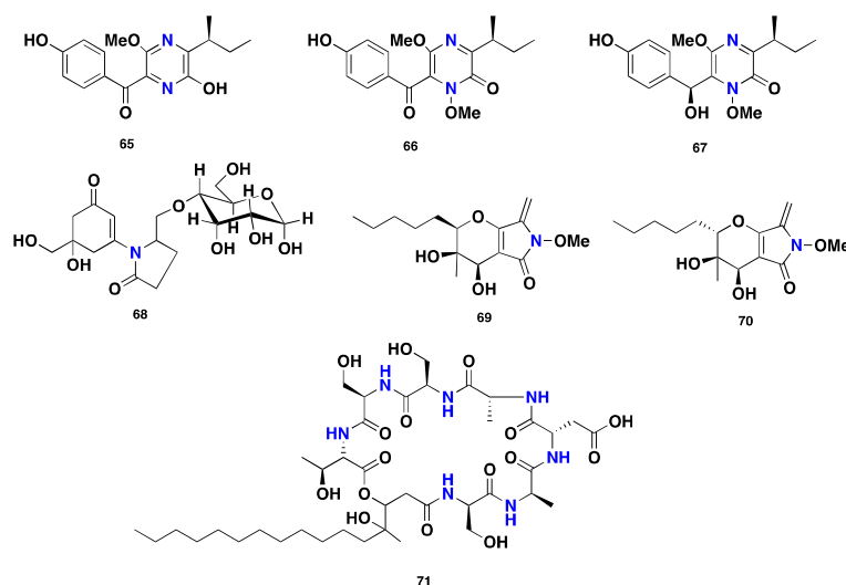
Figure 7. Chemical structures of 65–71.
