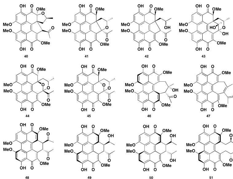
Figure 5. Chemical structures of 40–51.
