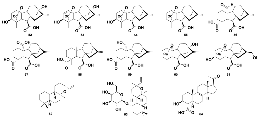
Figure 6. Chemical structures of 52–64 .
