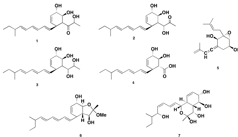
Figure 1. Chemical structures of 1–7.
