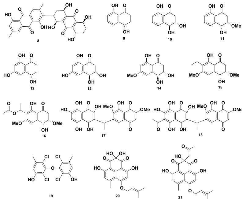
Figure 2. Chemical structures of 8–21.
