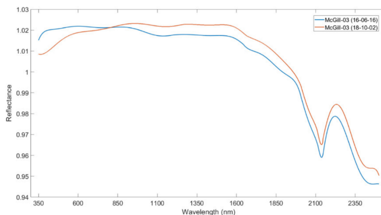
Figure 6. Degradation of the McGill-03 99% reflective Spectralon ® panel between two calibration dates (16 June 2016 and 2 October 2018).
