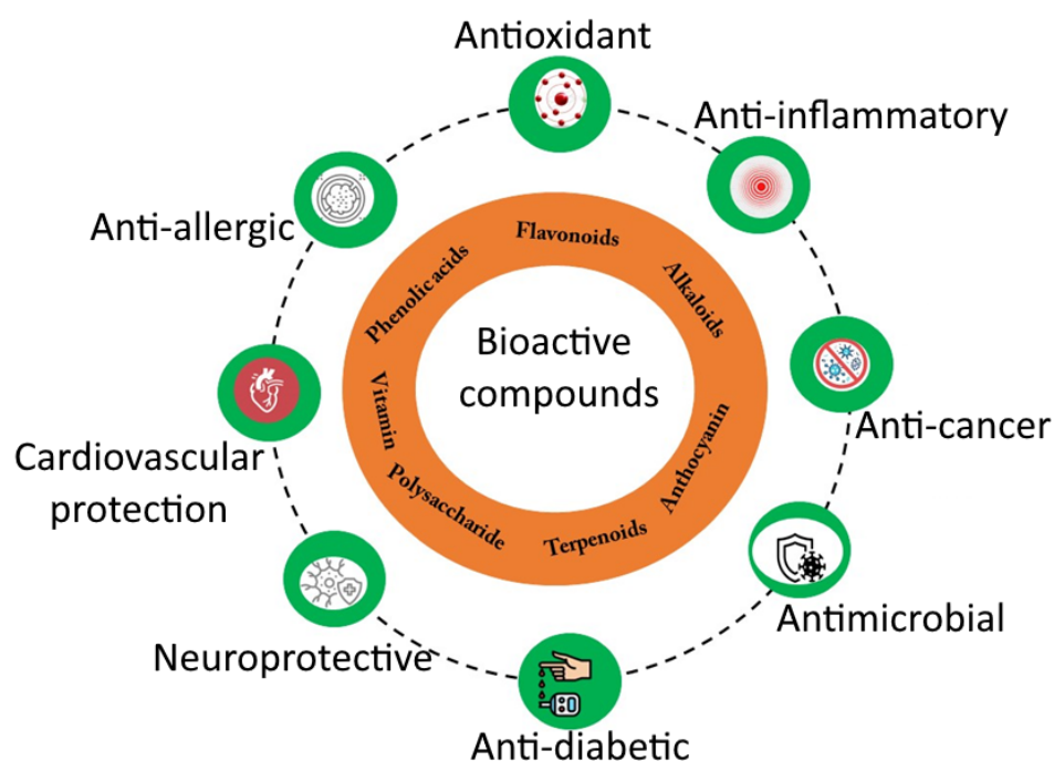
Figure 1. Bioactive compounds for different applications.
