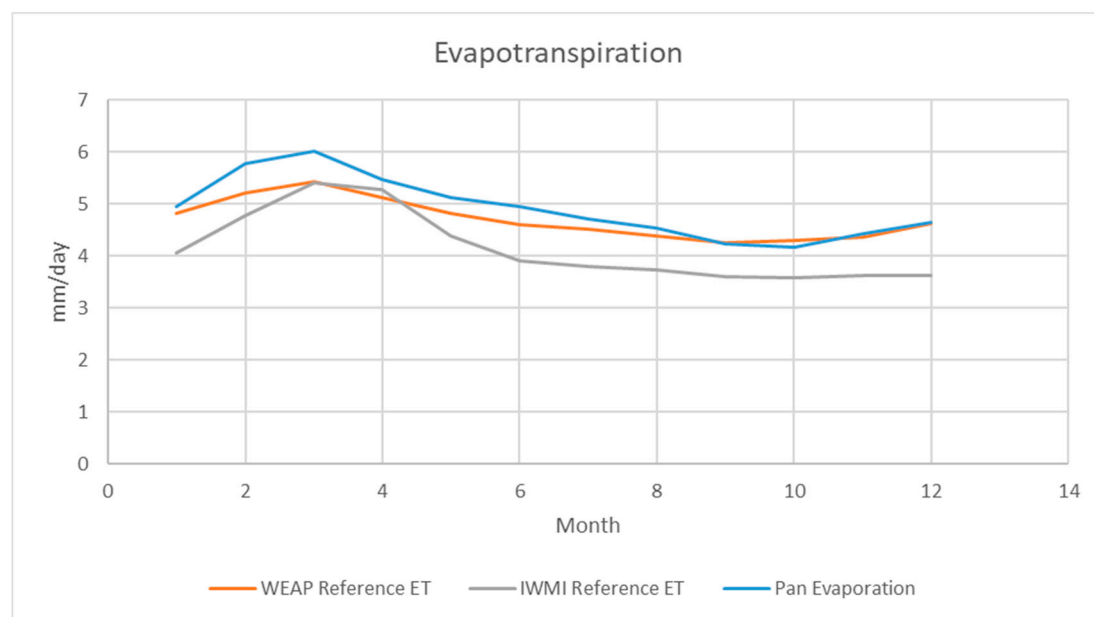
Figure 6. WEAP reference Evapotranspiration (ET) comparison with other estimates.
