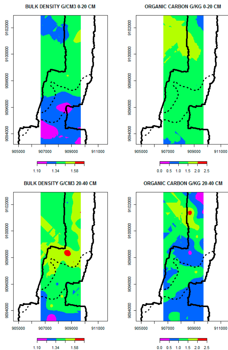
Figure 2. Spatial variation in bulk density, SOC along hydrological zones of transect derived from the geostatistical kriging method.
