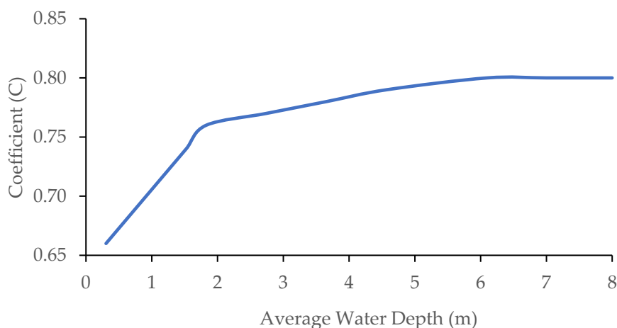
Figure 4. Surface Velocity coefficient as a function of water depth (USB, 2001).
