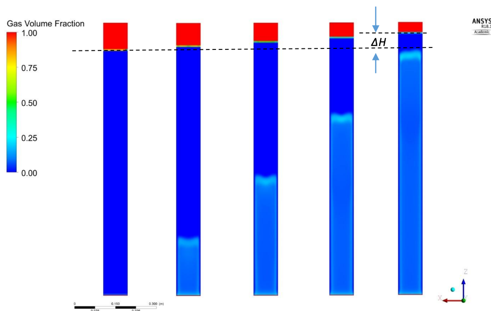
Figure 9. Bed expansion ( \Delta H ) for different time snapshots: t = 0, 0.8, 1.6, 2.4 and 3.2 s (air-water, U_{GS} = 0.2 m/s, d_p = 40 \mu m, d_c = 9 cm).
