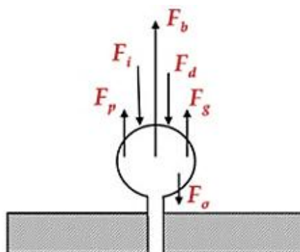
Figure 1. Forces acting on an under-formation bubble (Table 1).
