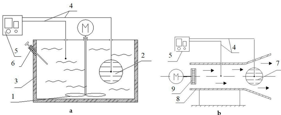
Figure 1. Setup for determining the thermal diffusivity and thermal conductivity coefficient of minced fish 1—stirrer; 2— \alpha -calorimeter; 3—liquid thermostat; 4—chromel-copel thermocouples; 5—microvoltmeter; 6—checking thermocouple; 7— \lambda -calorimeter; 8—airswitch; 9—fan.
