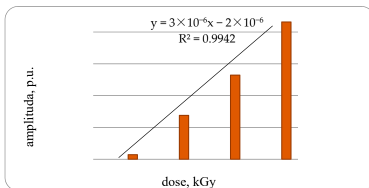
Figure 2. Amplitude of Electron Paramagnetic Resonance (EPR) signals samples of bone tissue of rainbow-cooled trout irradiated with different doses.
