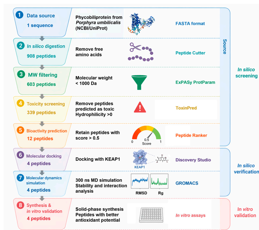
Figure 1. Graphical workflow of the integrated screening strategy for antioxidant peptides derived from phycobiliproteins of Porphyra umbilicalis .
