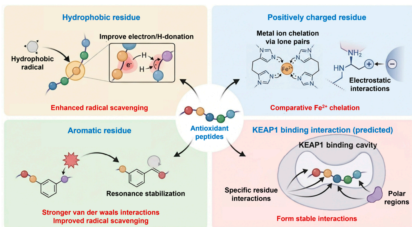
Figure 8. Schematic illustration of structure–activity relationship and intermolecular interaction mechanisms of antioxidant peptides.
