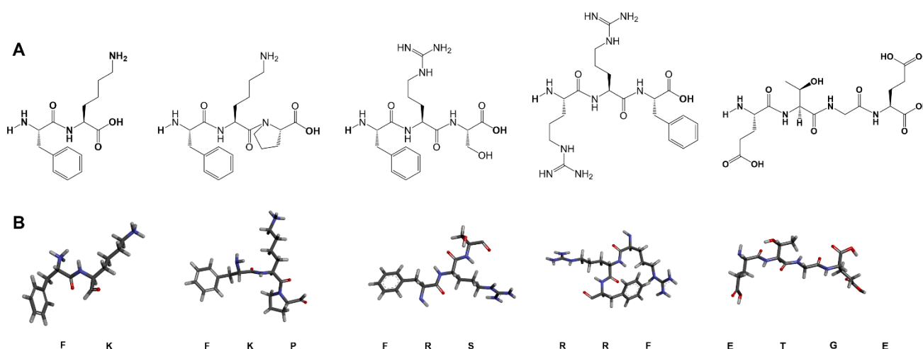
Figure 3. Chemical structures of candidate antioxidant peptides. (A) 2D structures; (B) 3D ball-and-stick models of FK, FKP, FRS, RRF and ETGE.
