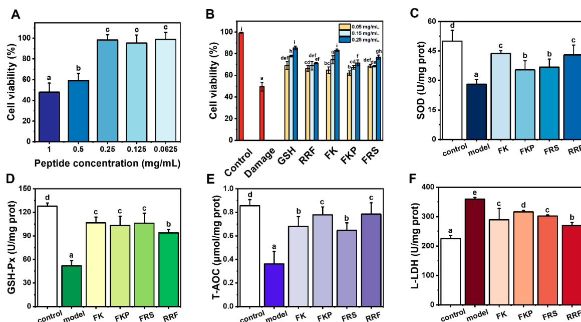
Figure 7. Protective effects of synthetic peptides against H_2O_2 -induced oxidative stress in Caco-2 cells. (A) Cell viability of Caco-2 cells after 24 h treatment with increasing concentrations of RRF (0.0625–1 mg/mL); (B) cell viability of H_2O_2 -damaged Caco-2 cells pretreated with the peptides at 0.05, 0.15, and 0.25 mg/mL; (C) superoxide dismutase (SOD) activity; (D) glutathione peroxidase (GSH-Px) activity; (E) total antioxidant capacity (T-AOC); (F) lactate dehydrogenase (LDH) release. Different lowercase letters indicate significant differences between groups ( P < 0.05 ).
