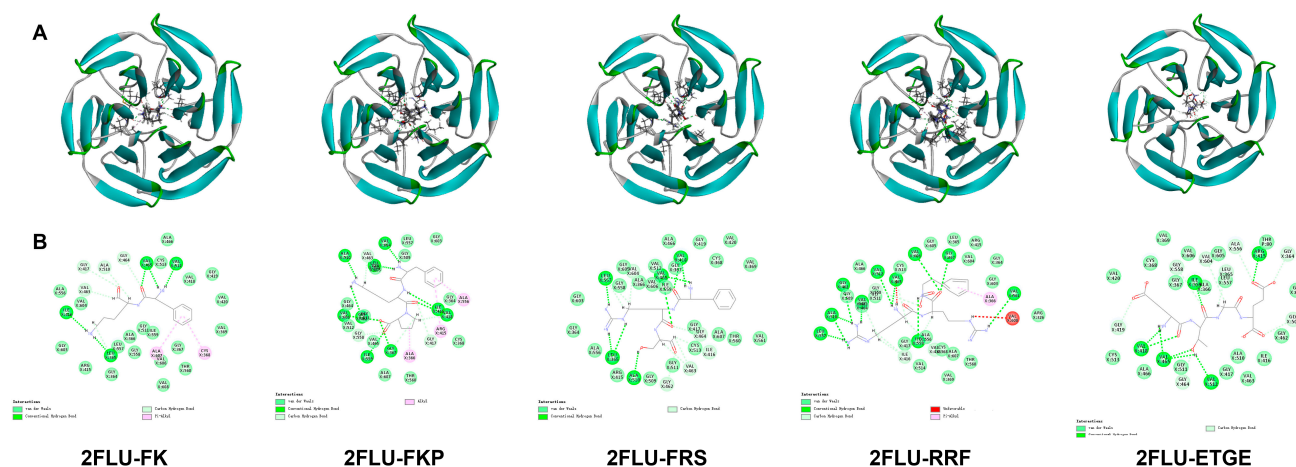
Figure 4. Molecular docking analysis of FK, FKP, FRS and RRF with KEAP1. (A) Docking conformations of peptides bound to KEAP1; (B) interaction force analysis between peptides and KEAP1.
