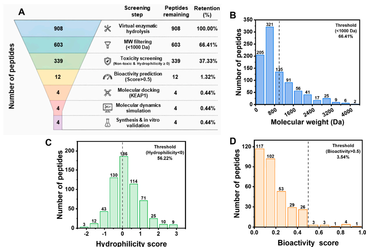
Figure 2. Statistical analysis of screening results and physicochemical properties of candidate peptides. (A) Number of peptides remaining after each screening step; (B) molecular weight distribution; (C) hydrophilicity value distribution; (D) bioactivity score distribution.
