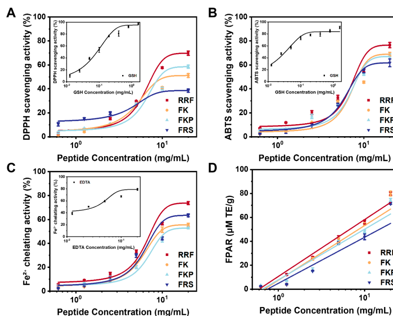
Figure 6. In vitro antioxidant activities of synthetic peptides. (A) DPPH radical scavenging activity; (B) ABTS radical scavenging activity; (C) \text{Fe}^{2+} chelating activity; (D) ferric reducing antioxidant power.
