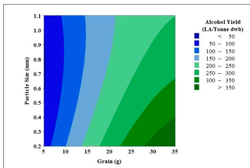
Figure 2. Contour plots showing the mean alcohol yields achieved during the response surface model, using varying grain amounts and grain particle sizes.
