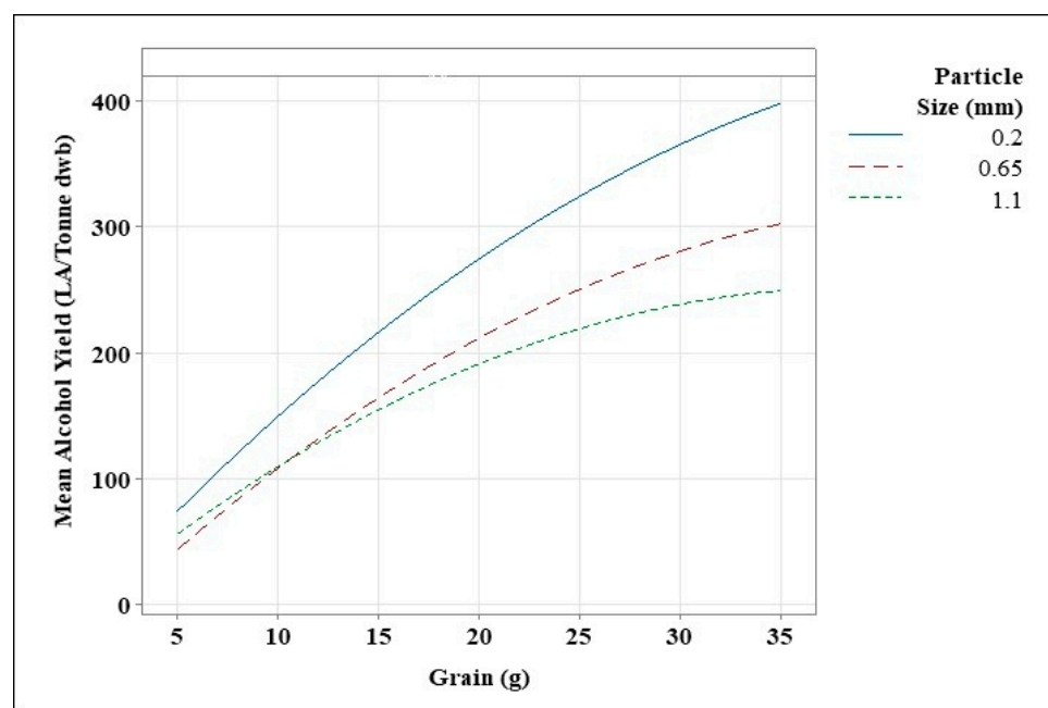
Figure 6. Interaction plots display the effect that both grain amount and grain particle size have on alcohol during the response surface model. This graph shows that a grain particle size of 0.2 mm at 35 g of grain will produce the highest yield.
