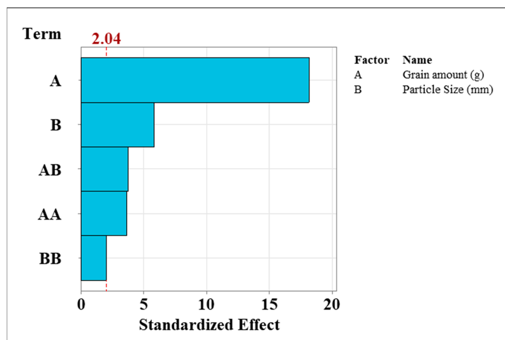
Figure 3. Pareto charts examining the standardised effects of the dependent variable (alcohol yield) on the independent variable (grain amount and size). All dependent variables above the 2.04 line
