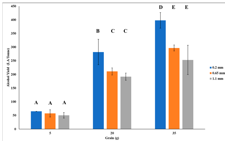
Figure 1. Mean alcohol yield achieved using different grain amounts and grain particle sizes. Results are presented as mean ( n = 3 ) and error bars indicating standard deviation. The same letter indicated no significant differences, as determined by one-way ANOVA with the Tukey post hoc test.
