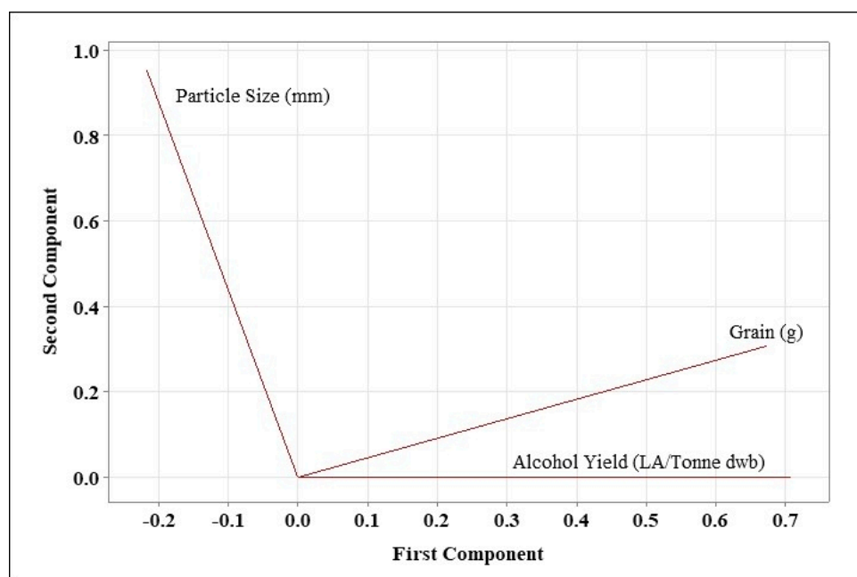
Figure 4. Principal component analysis of the dependent (alcohol yield) and independent variables (grain amount and particle size) used in this study. The amount of grain used has the biggest impact on AY, due to the closeness of the lines for alcohol yield and grain amount.
