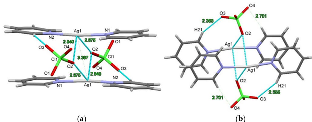
Figure 2. The centrosymmetric dimer of [\text{Agpy}_2\text{ClO}_4]_2 (a) and the \text{C}\alpha\text{-H}_{(\text{pyridine ligand})}\cdots\text{O}_{(\text{perchlorate})} interactions (b) in the dimer of compound 1.
