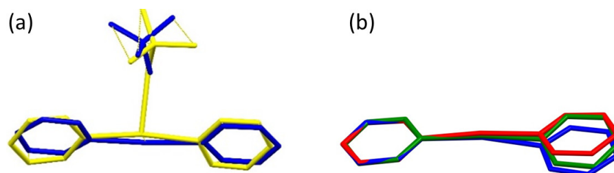
Figure 3. Comparison of (a) [\text{Agpy}_2]\text{ClO}_4\cdot 0.5\text{py} (compound 1) in blue and [\text{Agpy}_2]\text{MnO}_4\cdot 0.5\text{py} (compound 2) in yellow; (b) [\text{Agpy}_2]\text{ClO}_4\cdot 0.5\text{py} (compound 1) in blue, [\text{Agpy}_2]\text{ClO}_4 (compound 3) in red, and [\text{Agpy}_4]\text{ClO}_4\cdot 4[\text{Agpy}_2]\text{ClO}_4 (compound 4) in green.
