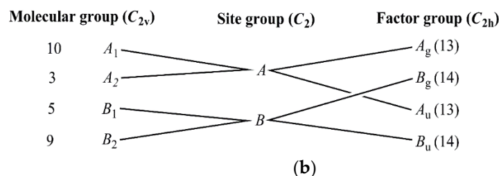
Figure 8. Correlation table for the 27 internal vibrational modes of the coordinated type of pyridine rings at C_1 (a) and C_2 (b) sites.
