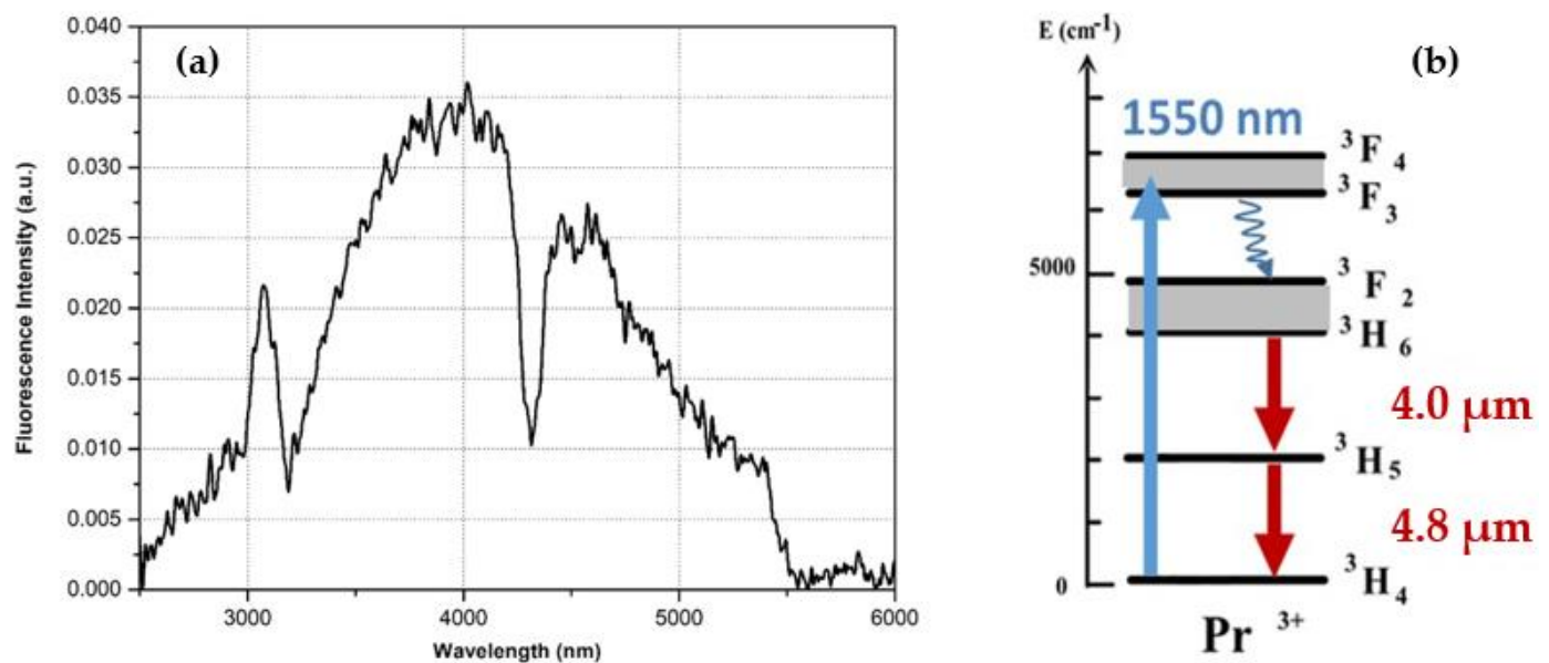
Figure 5. (a) Fluorescence intensity of the core of the double index fiber glasses ( [\text{GeS}_2]_{0.80}-[\text{Ga}_2\text{S}_3]_{0.20}90-(\text{CsCl})_{10} and [\text{GeS}_2]_{0.80}-[\text{Ga}_2\text{S}_3]_{0.20}90-(\text{CdI}_2)_{10}:1000 ppmw \text{Pr}^{3+} ) as a function of the wavelength; (b) energy level diagram of ion \text{Pr}^{3+} .
