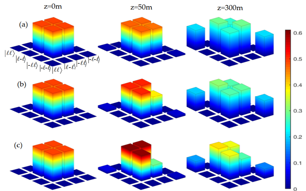
Figure 4. Graphic representations of the density matrices. The diagonal elements of the density matrices are horizontally arranged. (a) for l=3, p=0 ; (b) for l=3, p=1 ; (c) for l=3, p=2 .
