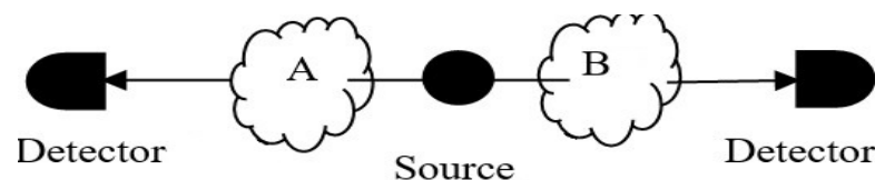
Figure 1. Sketch of the setup. A pair of entangled photons are generated by a source, and propagate along two weakly turbulent atmospheres which is labeled by A and B toward two detectors.
