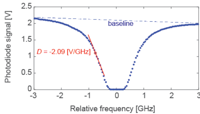
Figure 2. Example of \text{N}_2\text{O} absorption line used as a frequency discriminator to measure the FM response of the QCL. The P11e line of the vibrational band \nu_1 of \text{N}_2\text{O} located at 1275.5 \text{ cm}^{-1} was used in this case and is shown here. The absorption spectrum was measured by tuning the QCL or IH current and recording the voltage of the photodiode at the output of the reference gas cell. The current axis was converted into a relative frequency using the separately measured tuning coefficient. The operating point is shown by the red circle and the linear range by the red line with a slope D .
