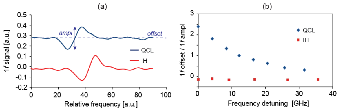
Figure 10. (a) Comparison of the first harmonic WMS signal of a \text{N}_2\text{O} line obtained for QCL injection current and IH current modulation (at T \approx 20^\circ\text{C} and I_{\text{QCL}} \approx 420\text{ mA} ), showing the strongly reduced background offset obtained for IH current modulation; (b) ratio between the offset and the amplitude of the 1f signal obtained for QCL and IH modulation at different QCL (IH) currents, converted into a corresponding frequency detuning. For each value of the QCL (IH) current, the laser temperature was slightly varied to keep the laser frequency around the considered \text{N}_2\text{O} transition. At each DC current, the amplitude of the applied modulation was adjusted to maximize the peak-to-peak amplitude of the 1f signal.
