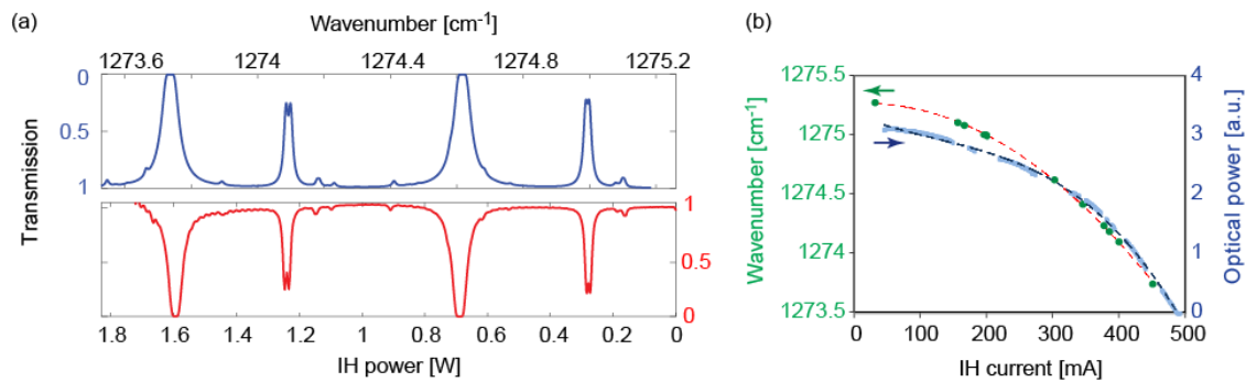
Figure 3. (a) \text{N}_2\text{O} absorption spectrum measured by tuning the QCL with the electrical power dissipated in the IH (bottom spectrum obtained at T = 25^\circ\text{C} and I_{\text{QCL}} = 450 \text{ mA} ) and corresponding \text{N}_2\text{O} absorption spectrum calculated from HITRAN database [13] for a \text{N}_2\text{O} pressure of 10 mbar diluted in air (total pressure of 70 mbar) over a pathlength of 10 cm (upper spectrum). The reference spectrum is inverted for the clarity of the figure. The total pressure in the reference cell that resulted from air contamination arising from the imperfect cell tightness was estimated to be \sim 70 \text{ mbar} from comparisons between measured and calculated spectra; (b) corresponding static tuning curve as a function of the IH current (green markers: experimental points; red dashed line: quadratic fit) and associated variation of the optical power (blue markers: Experimental points; blue dashed line: 3rd order polynomial fit). The experimental data of the optical power were extracted from the measured transmission through the \text{N}_2\text{O} cell; the gaps in the data result from the presence of \text{N}_2\text{O} absorption lines that have been removed.
