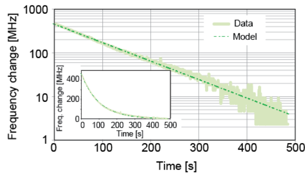
Figure 6. Temporal evolution of the QCL optical frequency measured for a step change of the TEC temperature of \sim 0.16 K, displayed in a semi-log scale. The inset shows a linear representation. The experimental data are well approximated by a single exponential decay with a time constant of \sim 100 s (dashed-dotted line).
