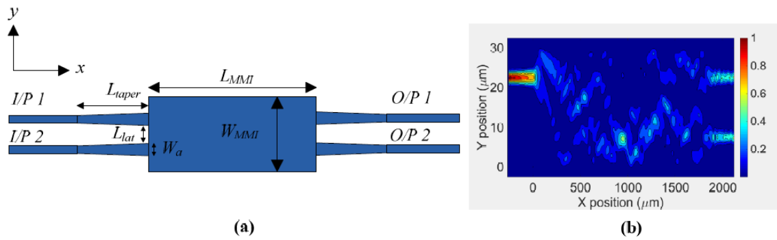
Figure 3. (a) Schematic of the 2 \times 2 multimode interference (MMI) coupler with taper waveguide length, L_{taper} = 200 \mu\text{m} and access waveguide width, W_a = 5 \mu\text{m} and (b) the electric field distribution in a 2D plane of the MMI coupler at 1550 nm wavelength.
