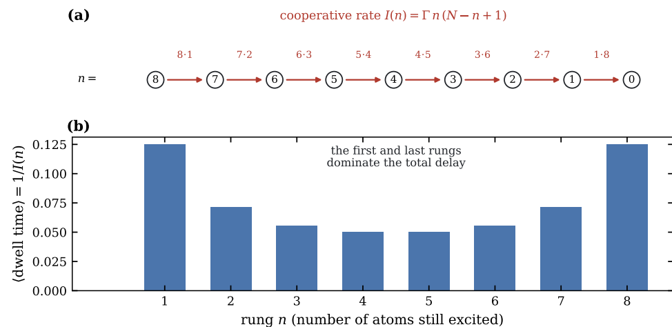
Figure 1. The Dicke ladder as a one-way random walk, with N = 8 . (a) The cooperative rate I(n) = \Gamma n(N - n + 1) is largest in the middle of the chain and smallest at the two ends. (b) The mean dwell time 1/I(n) on each rung. The delay in the burst is the sum of the dwell times over the upper half of the chain, and this sum is dominated by the first few rungs: the ensemble waits for the first few photons and then avalanches.
