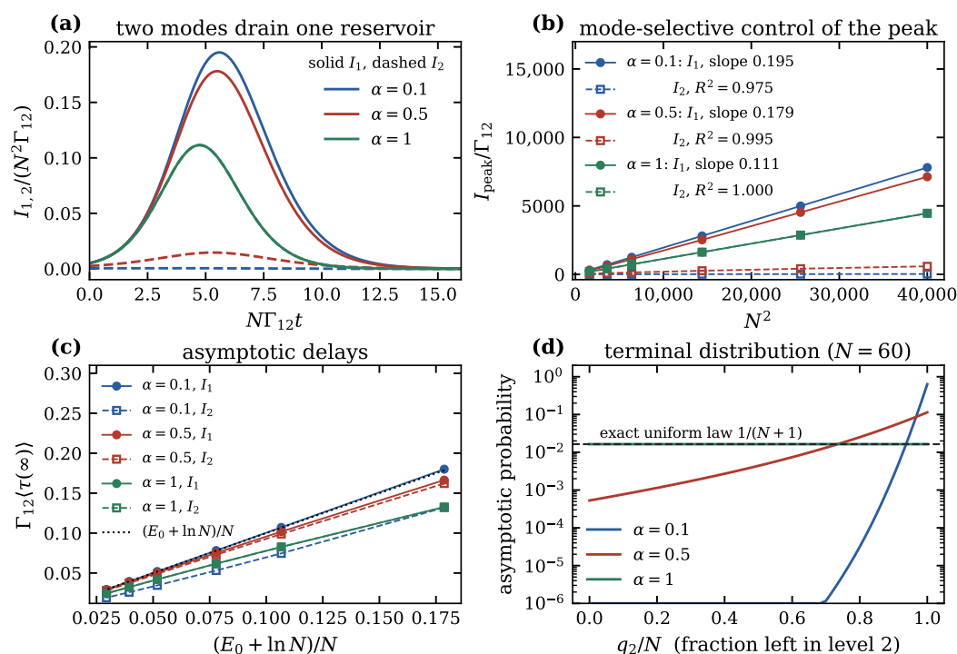
Figure 6. The shared-source configuration; panels (a–c) correspond to Ref. [19], and panel (d) was computed for this review from Equation (7) (cf. Ref. [59]). (a) Mode-resolved transients at N = 200 : The two channels drain one reservoir, so strengthening one weakens the other. (b) Peak intensity against N^2 : Mode 1's slope falls from 0.195 ( \alpha = 0.1 ) to 0.111 ( \alpha = 1 ), constituting the mode-selective control effect. (c) Asymptotic running delays. (d) Final distribution over the absorbing bottom edge: It is exactly uniform at \alpha = 1 (dashed line) and increasingly one-sided as \alpha decreases.
