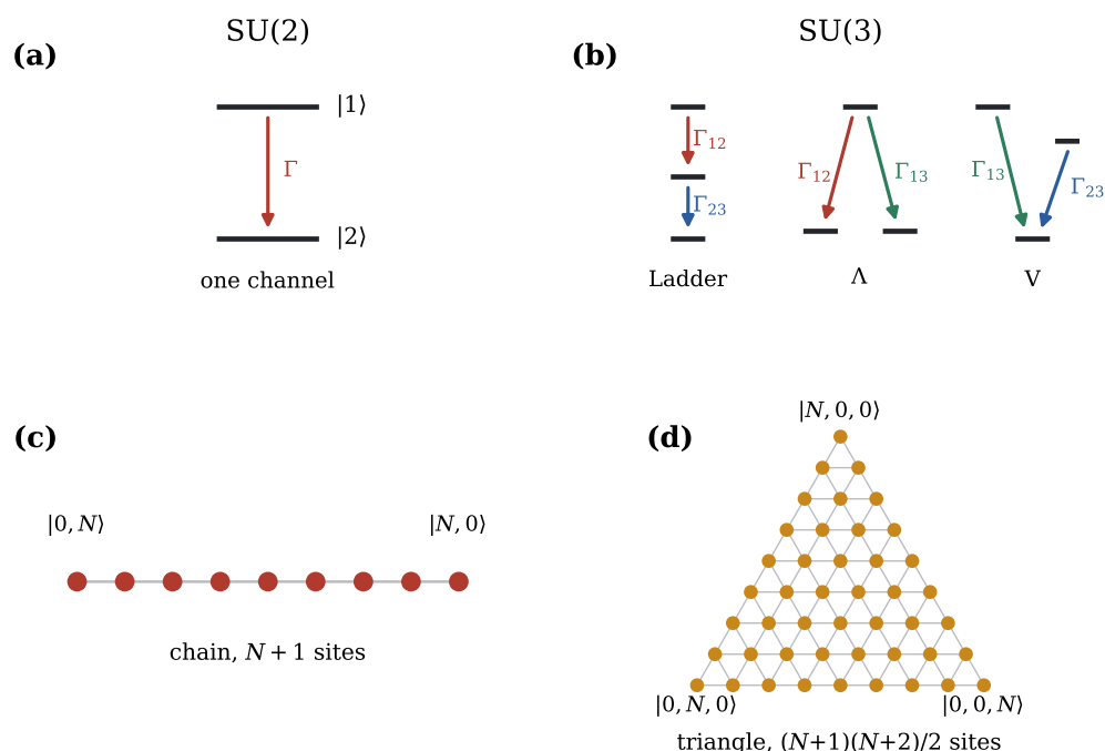
Figure 3. (a) The two-level atom and its single channel. (b) The three dipole-allowed three-level configurations covered in Section 4: cascade, shared-source, and shared-sink. (c,d) The corresponding occupation-number lattices at N = 8 : a chain of N + 1 sites and a triangle of \frac{1}{2}(N + 1)(N + 2) sites. Four-level atoms occupy a tetrahedron [23].
