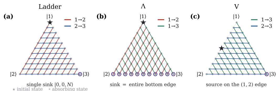
Figure 4. The three dipole-allowed three-level configurations as bond sets on the triangular occupation-number lattice ( N = 10 ). Grey bonds are lattice directions closed by parity; colored bonds are open channels. Stars mark the initial states used in each paper reviewed below; open circles mark absorbing states (states the ensemble cannot leave). (a) Cascade: The two channels are in series, and the flow must cross the lattice from |N, 0, 0\rangle to |0, 0, N\rangle . (b) Shared-source: The two channels compete for the same source, and the absorbing set is the entire bottom edge. (c) Shared-sink: The natural initial state is the midpoint of the (1, 2) edge, and both channels end on the same vertex.
