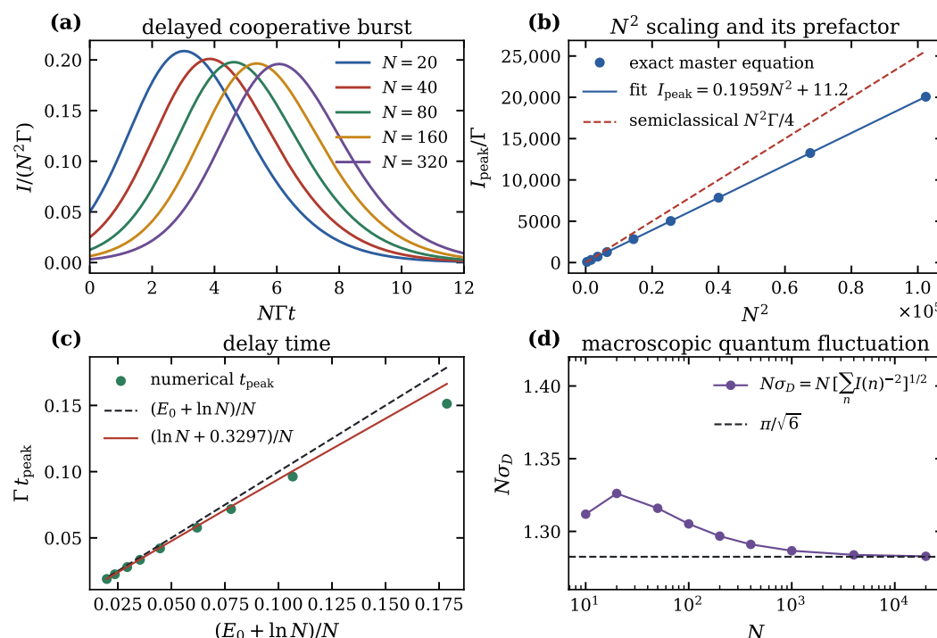
Figure 2. The two-level benchmarks. (a) Normalized bursts: rescaling time by N\Gamma collapses the curves, except for the slow logarithmic drift of the delay. (b) Peak intensity against N^2 , which is about 21.7% below the semiclassical dashed line N^2\Gamma/4 . (c) The time of the peak (dots), compared with the mean delay (E_0 + \ln N)/(\Gamma N) (dashed) and with (\ln N + 0.3297)/(\Gamma N) (solid), the peak time of the Gumbel-averaged \text{sech}^2 pulse. The peak comes earlier than the mean delay because the averaged pulse peaks between the most probable delay, \ln N/(\Gamma N) , and the mean delay. (d) The exact delay standard deviation, rescaled by N , approaching \pi/\sqrt{6} .
