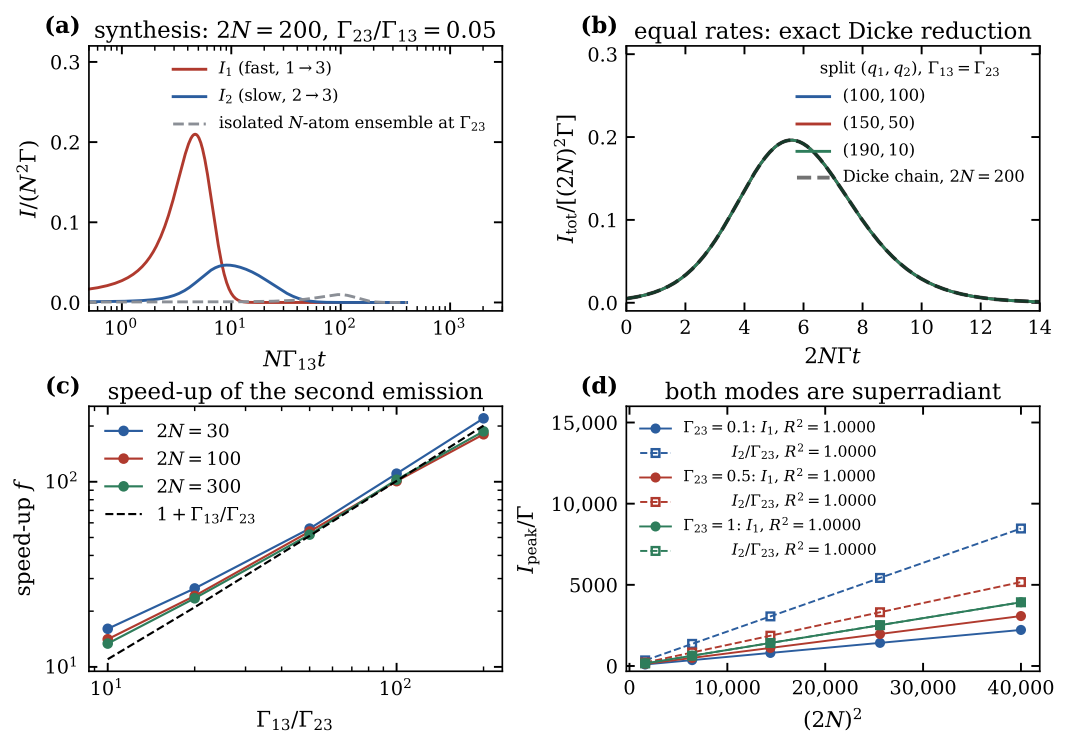
Figure 7. The shared-sink configuration and superradiant synthesis, as per Ref. [20]. (a) The slow mode fires immediately behind the fast one, which is an order of magnitude earlier than the same group of atoms would fire in isolation (dashed). (b) For equal rates, the total transient is exactly the 2N -atom two-level burst for every split of the atoms between the two excited levels. (c) The speed-up factor against the rate ratio. (d) Both modes obey the N^2 law throughout, unlike the shared-source case.
