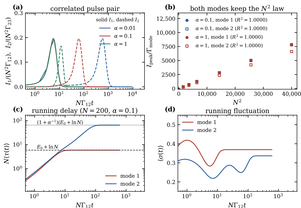
Figure 5. Cascade superradiance, as per Ref. [18]. (a) Mode-resolved transients for N = 200 : decreasing \alpha separates the pulse pair in time without changing either pulse’s shape. (b) Both modes obey the N^2 law. (c) Running delays: Mode 1 saturates at E_0 + \ln N and mode 2 at (1 + \alpha^{-1})(E_0 + \ln N) . (d) Running fluctuations: Mode 2’s two minima are the timing signature of a correlated pulse pair.
