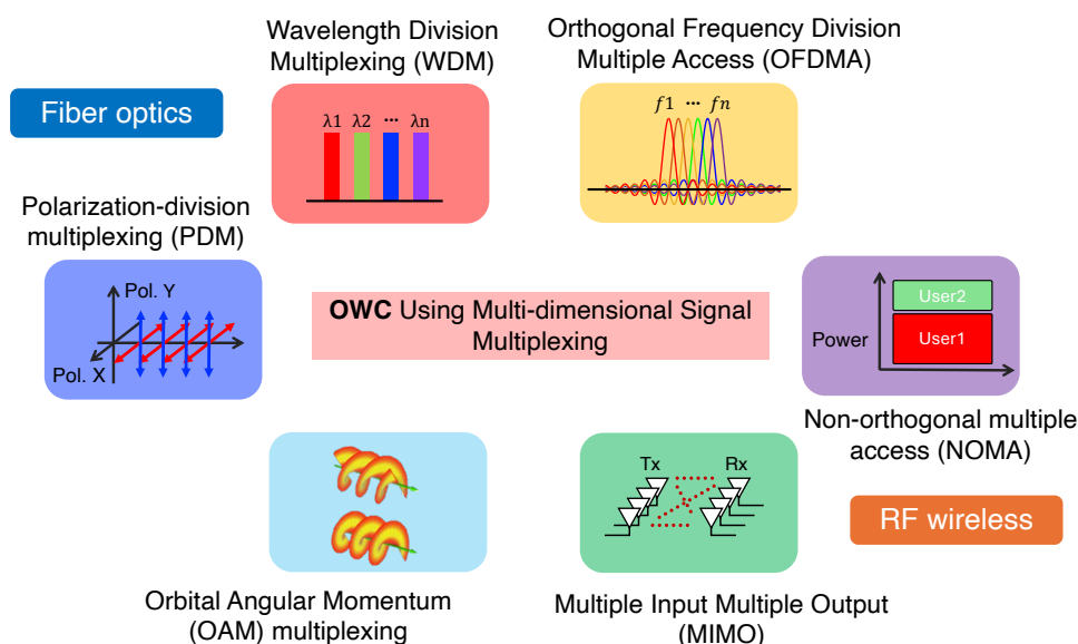
Figure 1. A wide range of transmission multiplexing techniques used in fiber optics and RF wireless communications can potentially be applied to OWC to achieve high-dimensional multiplexing.
