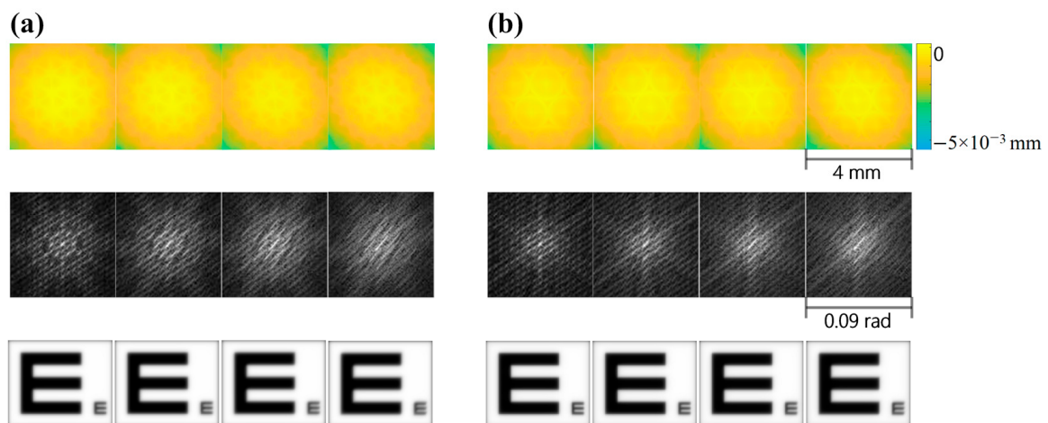
Figure 7. Imaging quality evaluation of (a) O-HOPE spectacle lens and (b) T-HOPE spectacle lens for increasing gaze angles, which are 13.3°, 19.5°, 25.2°, and 30.5° (from left to right). First row: Emergent wavefront. Second row: PSF. Third row: Simulated image of letter E.
