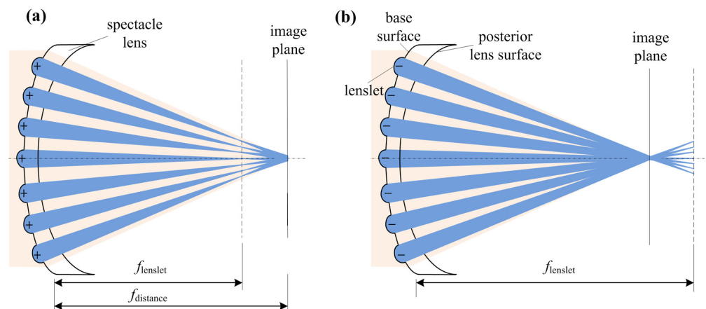
Figure 2. Schematic ray tracing of LARI spectacle lens with lenslets of +3.00 D addition power (a) and −3.00 D addition power (b), and lenslets form multiple separate focal point (lenslet with plus power focuses in front of distance focal plane and lenslet with minus power focuses behind distance focal plane). f_{\text{lenslet}} : focal length of lenslets, f_{\text{distance}} : focal length of spherical base surface.
