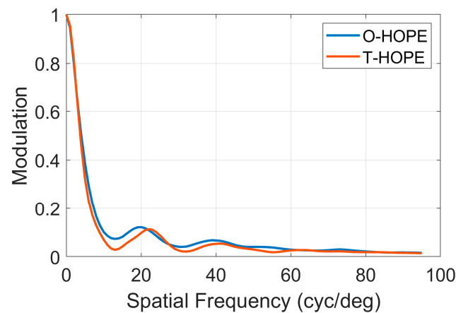
Figure 8. The calculated average MTF in the whole circumference direction of HOPE spectacle lens for the gaze direction featured by the chief ray position of (6, 6) on the lens surface, as defined in Figure 3, with a gaze angle of 19.5^\circ .
