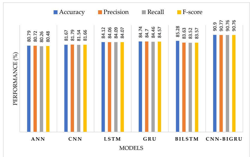
Figure 5. CNN-BiGRU model results using HES dataset.
