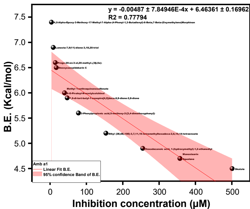
Figure 9. Inhibitory potency of NADES extract components toward (a) Cry j 1 and (b) Amb a 1. (left) Binding energy (B.E.) of docking and inhibition constant of each extracted component to the allergens and (right) their regression analysis.
