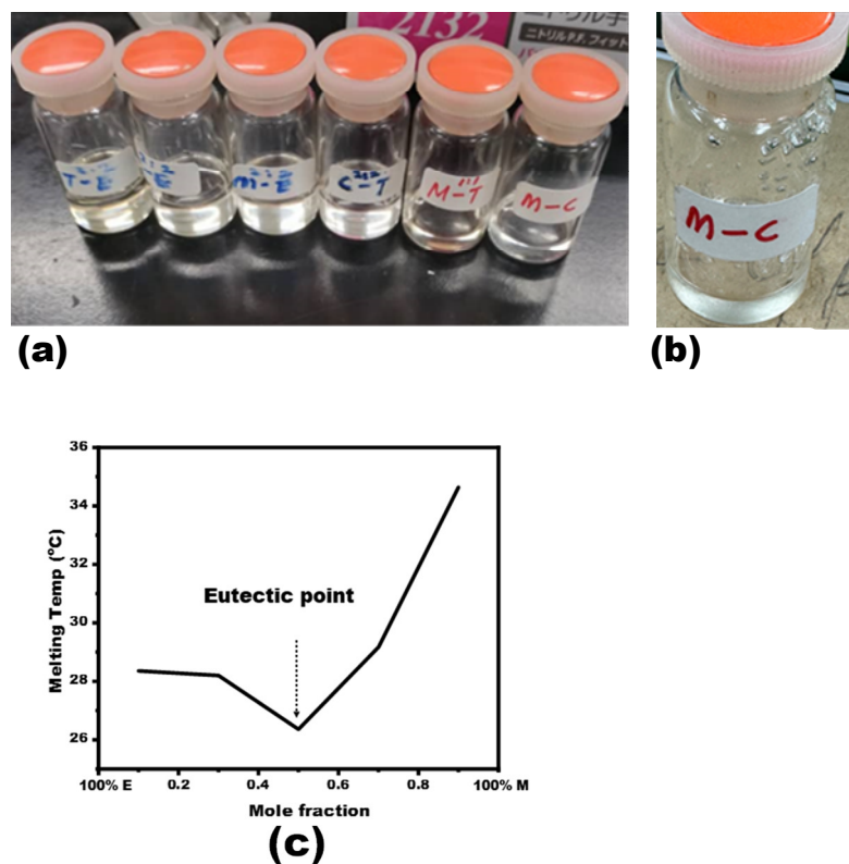
Figure 2. (a) Visuals of the synthesized NADESs. (b) After 4 days. (c) Solid–liquid phase diagram of menthol–eugenol NADES system based on DTA analysis. The plot shows the onset melting temperatures of mixtures at various molar ratios of menthol (mole fraction 0.1–0.9). The minimum point at the 1:1 molar ratio indicates the eutectic composition, confirming the formation of a stable NADES at this ratio.
