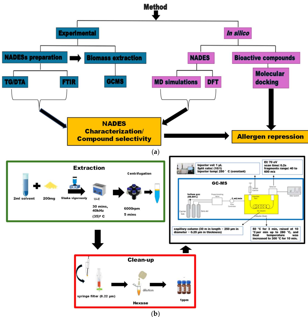
Figure 1. (a) Schematic flowchart of the current study; NADES preparation, characterization, extraction, and potential allergen-repressing investigation. (b) Flow chart illustrating the extraction procedure of bioactive compounds from Thujopsis dolabrata wood biomass using ultrasonic-assisted extraction, followed by GC–MS characterization for compound identification and profiling.
