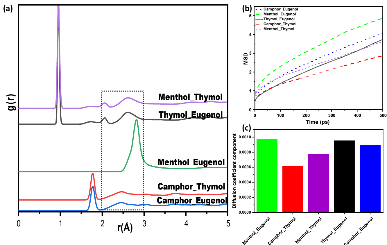
Figure 8. Molecular dynamics analysis of the simulated NADESs showing (a) atom–atom radial distribution functions (RDFs), (b) mean square displacement, and (c) diffusion coefficient components of the different natural deep eutectic solvents at 1 bar and 298 K.
