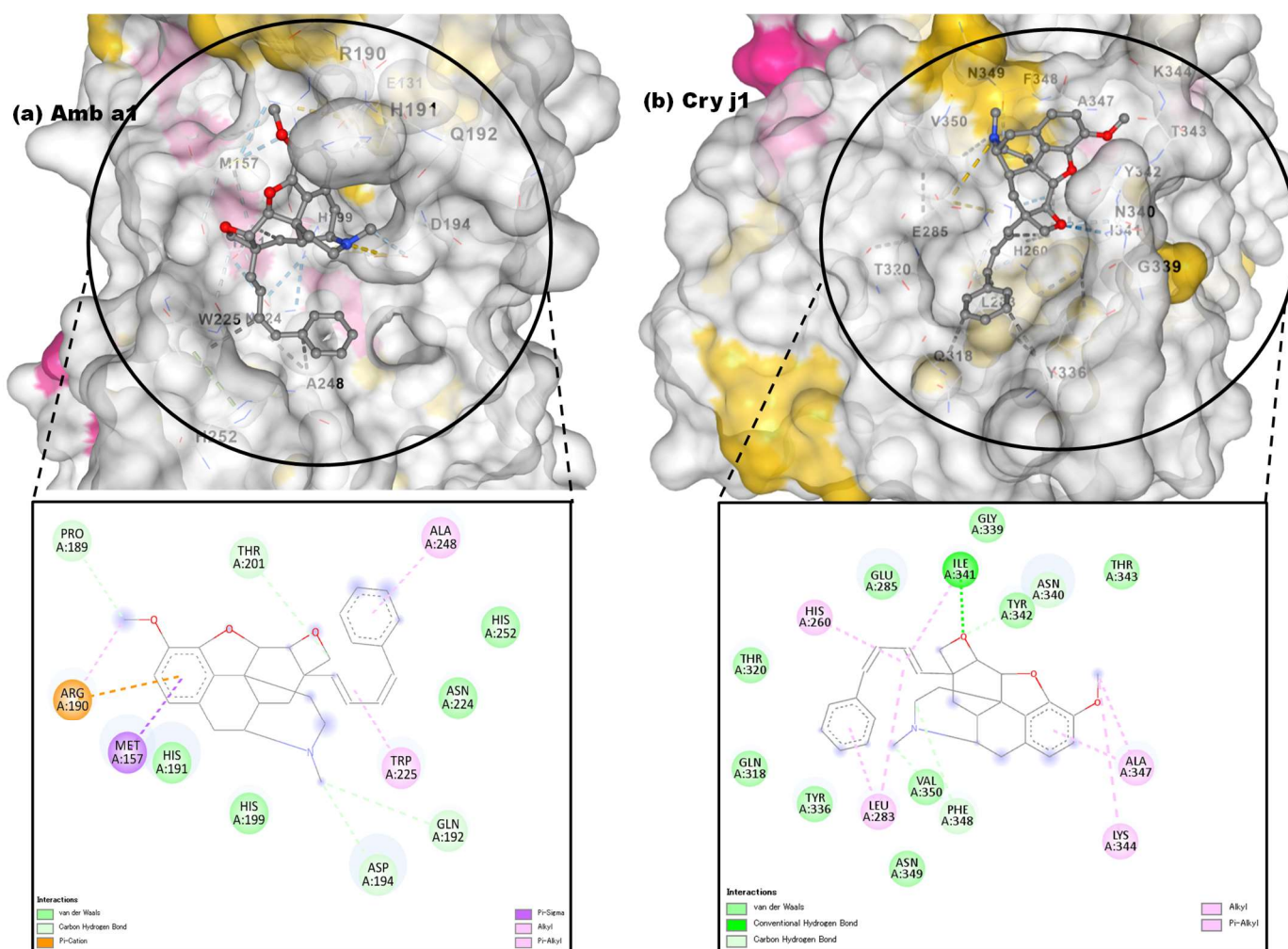
Figure 10. 2D and 3D visualization of the interaction between Methyl-7-Alpha-(4-Phenyl-1,3-Butadienyl)-6-Beta,7-Beta-(Oxymethylene) Morphinan and allergen protein: (a) Amb a 1, (b) Cry j 1.
