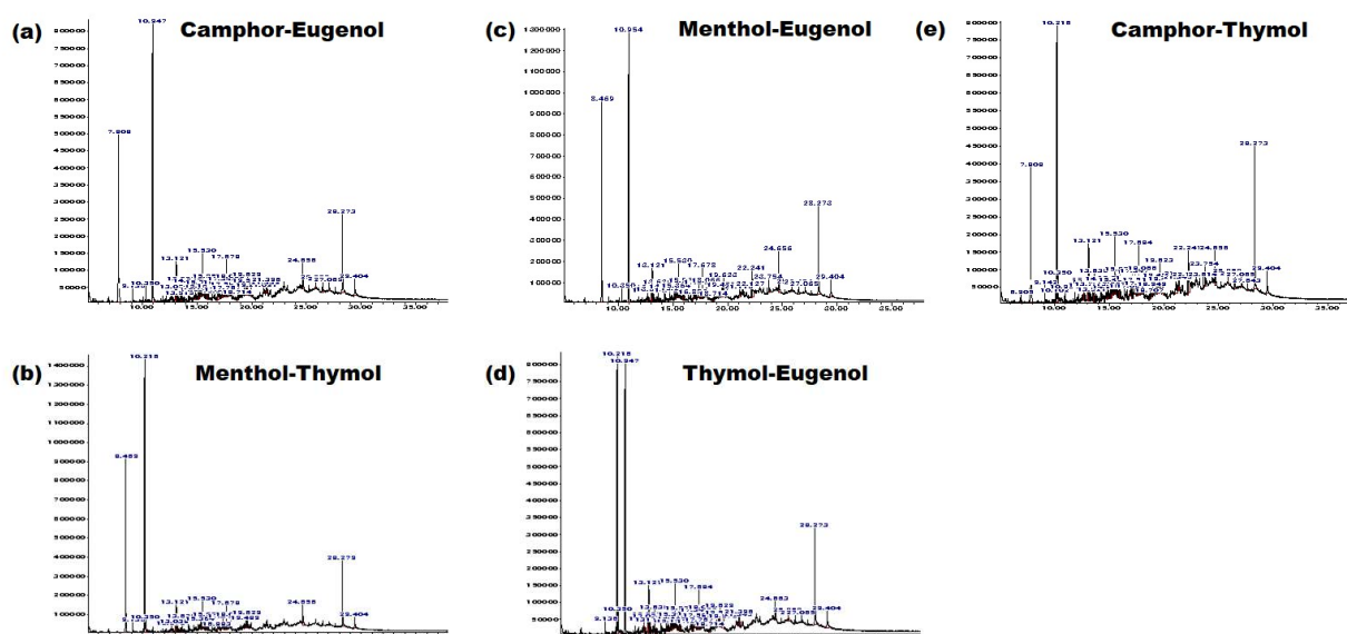
Figure 4. TIC obtained from the GCMS analysis of the hydrophobic NADES extract of T. dolabrata wood biomass: (a) camphor–eugenol, (b) menthol–thymol, (c) menthol–eugenol, (d) thymol–eugenol, (e) camphor–thymol.
