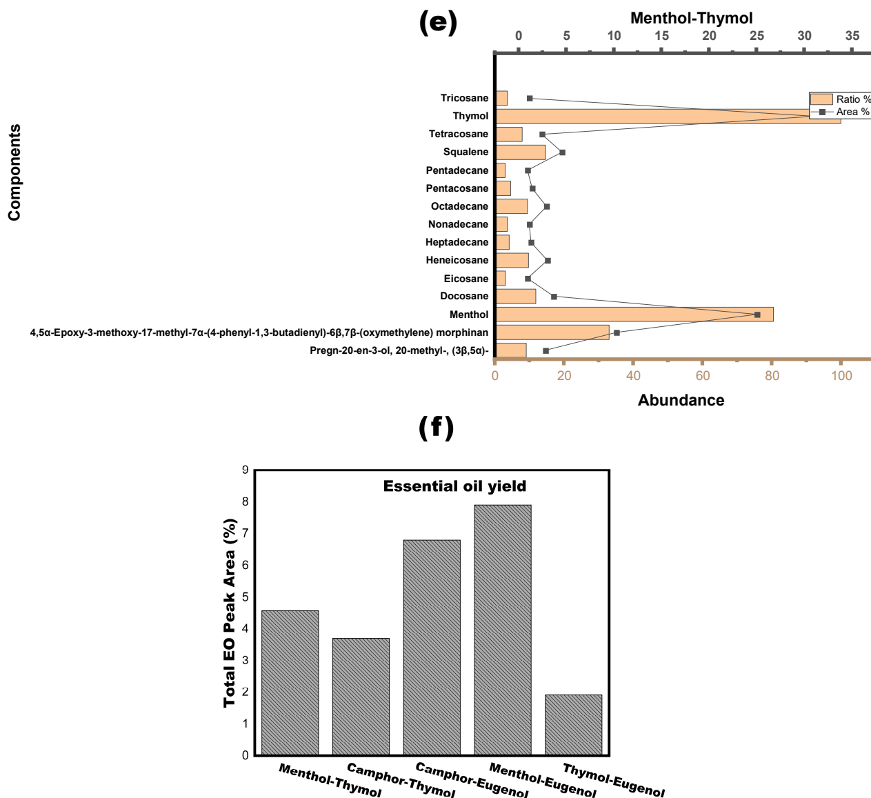
Figure 5. (a–e) The NADES extract compositions plotted as components against abundance (% peak area and ratio). (f) Semiquantitative comparison of essential oil content extracted using different NADES systems based on GC–MS peak area percentages. The total essential oil content was estimated by summing the peak area percentages of four key essential oil compounds—ethyl (2E,6E,10E)-3,7,11,15-tetramethylhexadeca-2,6,10,14-tetraenoate, deoxycasaldekarin C, lanosta-7,9(11)-diene-3,18,20-triol, and squalene identified in each extract. Values represent the relative abundance of these compounds within the total ion chromatograms of each NADES extract.
