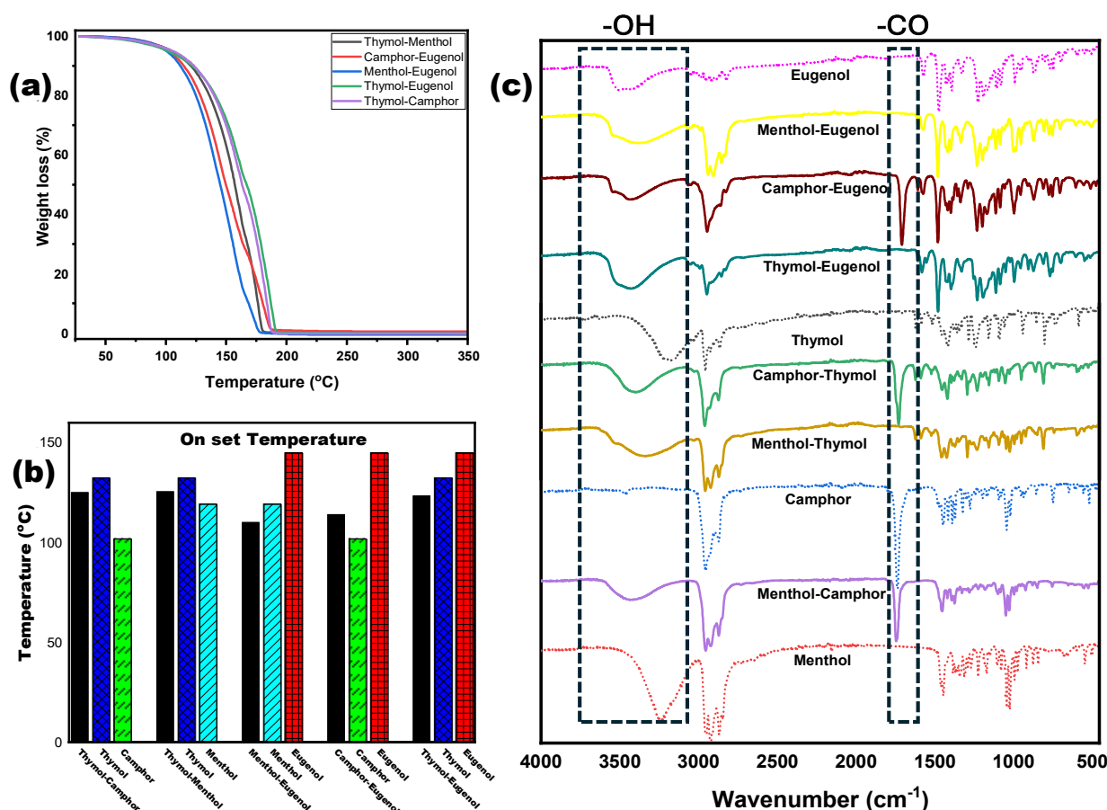
Figure 3. (a) TGA curves of the NADESs. (b) Comparison between the T_{\text{onset}} (onset temperature) of the NADESs and the pure components. (c) FTIR spectra of the NADESs and the pure components.
