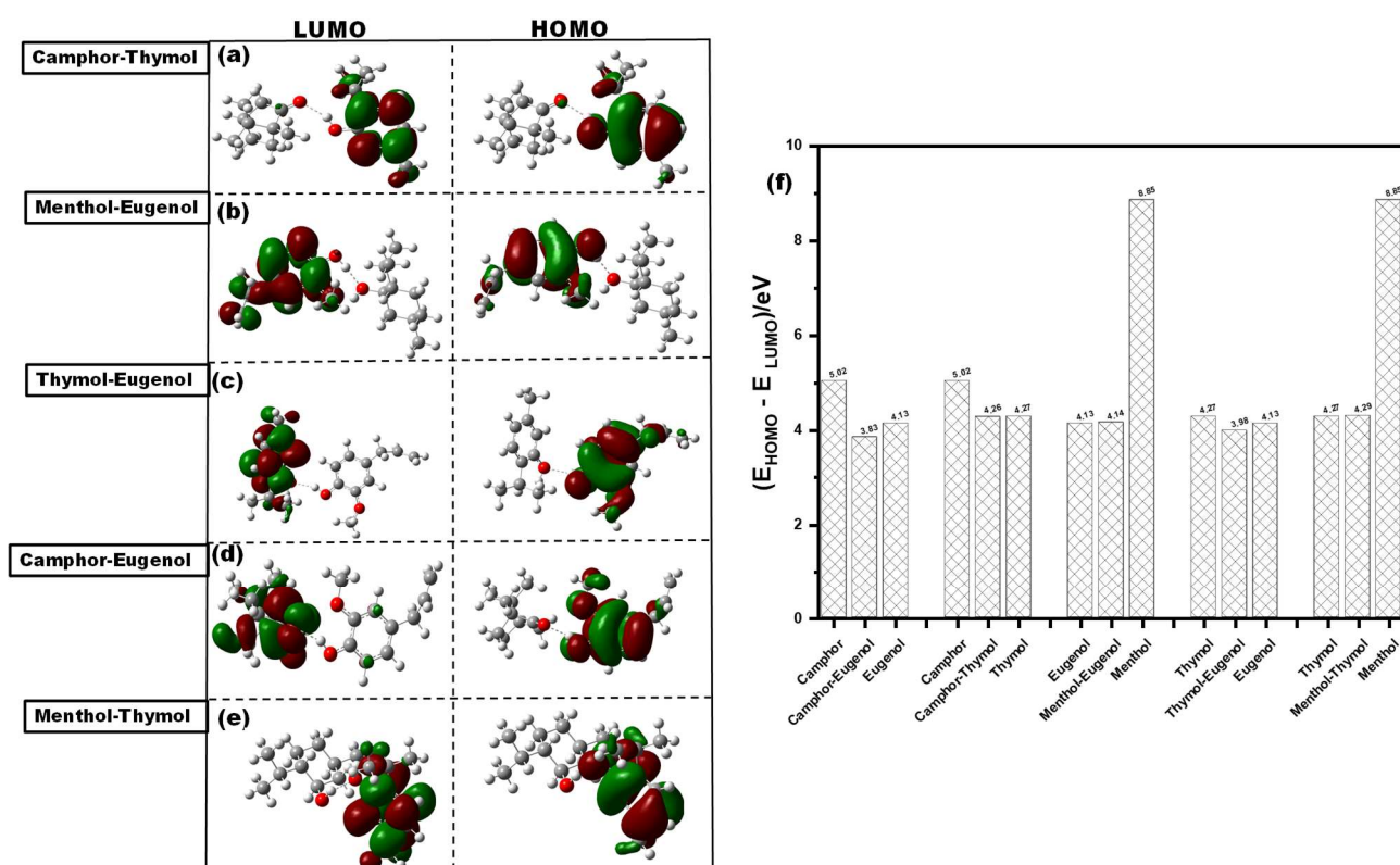
Figure 6. (a–e) The HOMO-LUMO structure diagrams of the simulated NADESs. (f) Plot of the energy difference of the HOMO-LUMO of the pure components and the NADESs.
