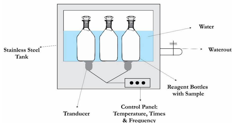
Figure 2. Ultrasonic bath mode.
