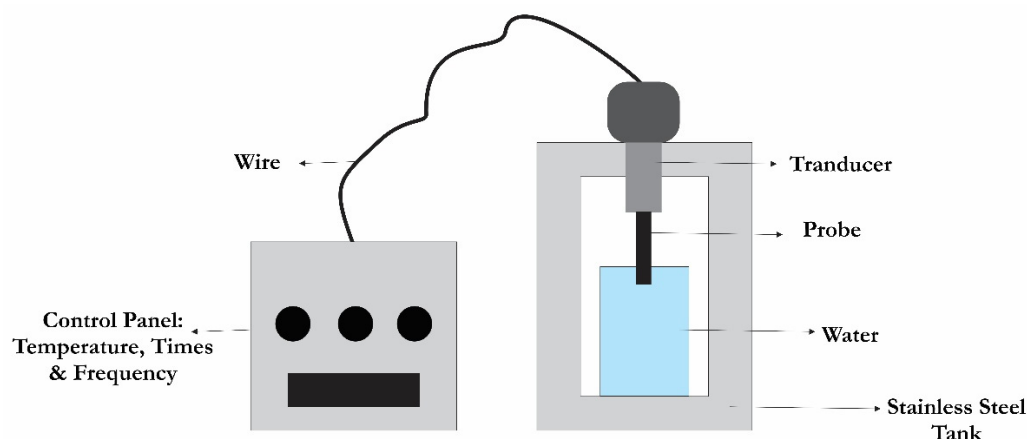
Figure 3. Ultrasonic probe mode.
