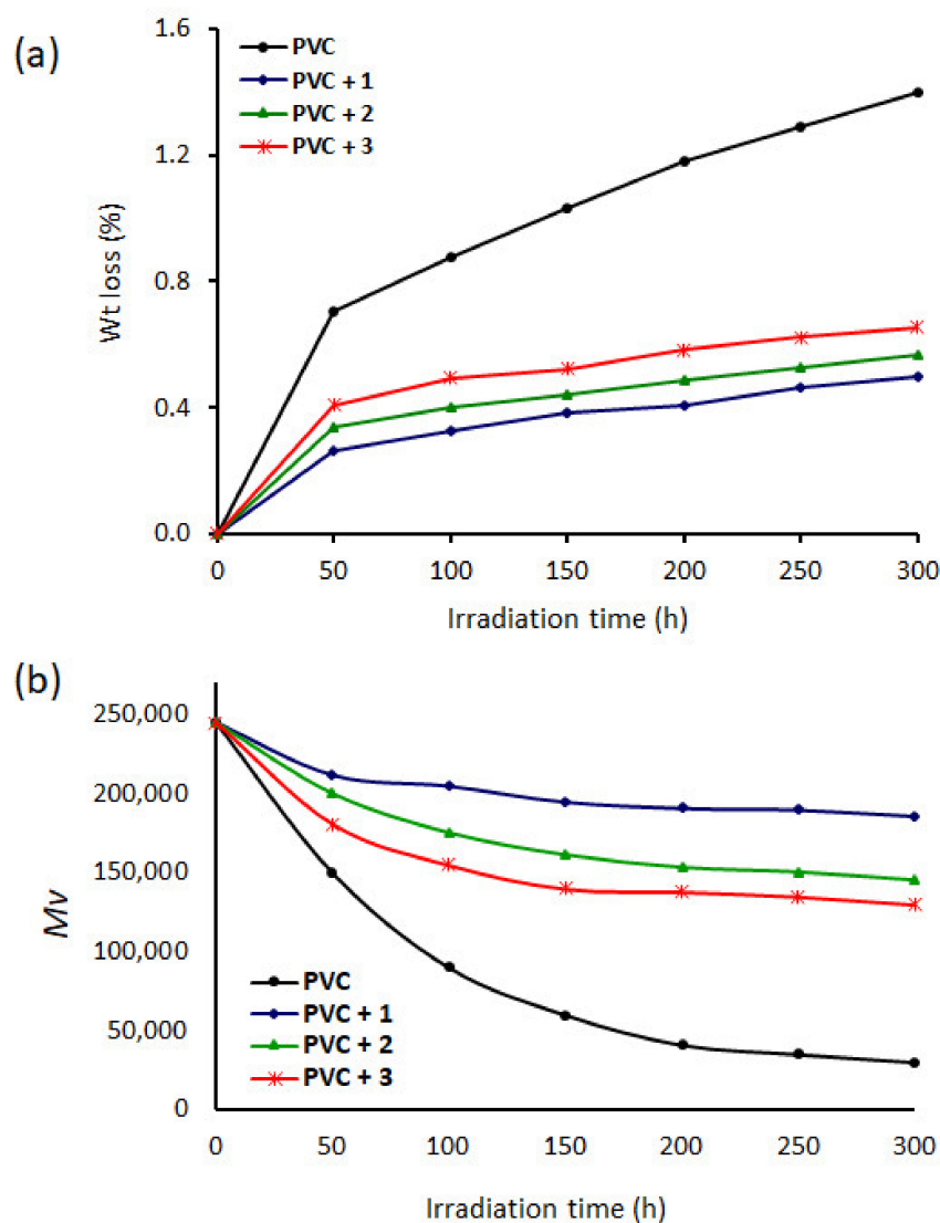
Figure 3. Effect of organosilanes 1–3 on the (a) weight loss (%) and (b) \overline{M}_V of PVC.
