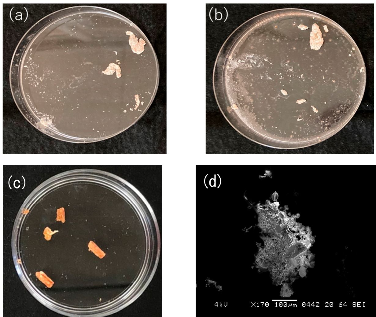
Figure S1. Images of Lf loaded shellac microparticle-agglomeration by PGSS process at (a) 20 °C, (b) 30 °C, and (c) 50 °C, at 10 MPa. SEM images of shellac (sole) microparticles produced by PGSS process at 10 MPa and at 50 °C (d).
