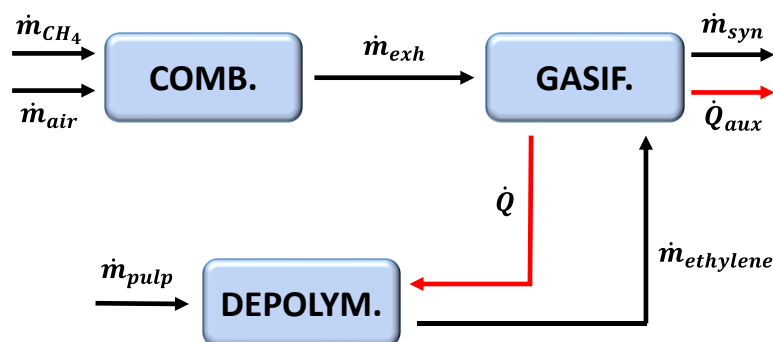
Figure 4. Thermochemical scheme of the MR pyro-gasification plant.
