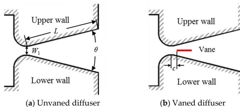
Figure 2. Geometries of test diffusers.
