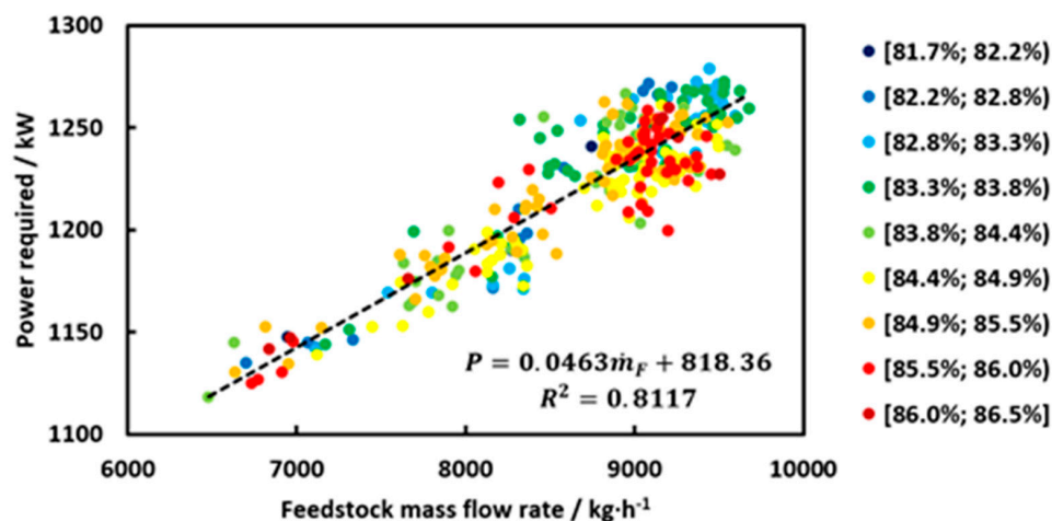
Figure 10. Process side characteristics.
