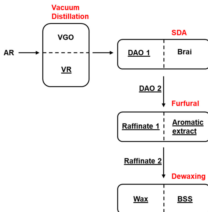
Figure 1. Lubricant oil production scheme.
