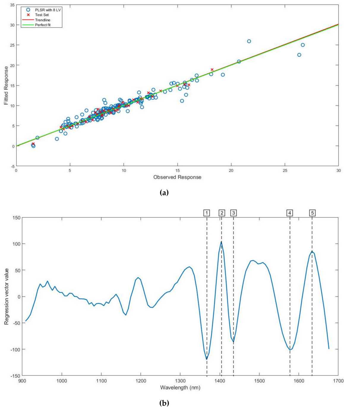
Figure 3. (a) Partial least squares regression plot for the prediction of BWC on WD_{gr} . Raw spectra were pre-processed with no pretreatments using eight latent variables; (b) Corresponding regression vector plot using vertical lines and numbers to highlight the most important wavelengths.
