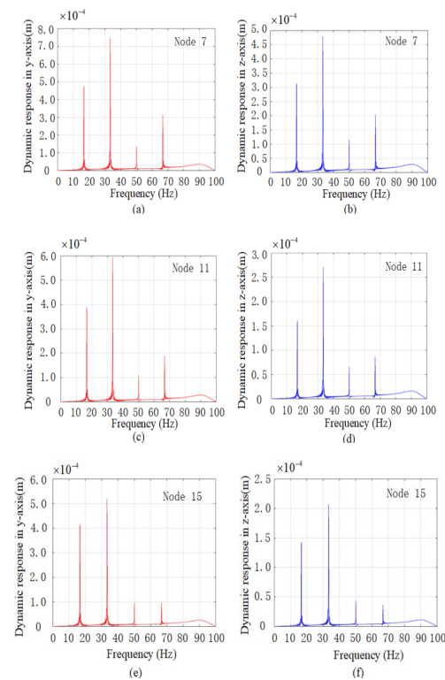
Figure 14. The mathematical simulated dynamic response with 0.8 mm parallel misalignment and 0.5^\circ angular misalignment of nodes 7, 11, and 15 in the y -axis and z -axis. (a) Node 7 in the y -axis. (b) Node 7 in the z -axis. (c) Node 11 in the y -axis. (d) Node 11 in the z -axis. (e) Node 15 in the y -axis. (f) Node 15 in the z -axis.
