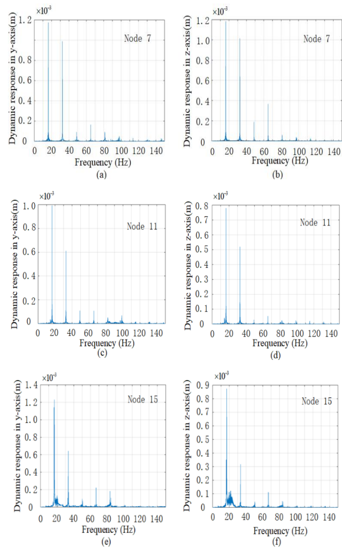
Figure 19. The experimental dynamic response with 0.8 mm parallel misalignment and 0.5^\circ angular misalignment of nodes 7, 11, and 15 in the y-axis and z-axis. (a) Node 7 in the y-axis. (b) Node 7 in the z-axis. (c) Node 11 in the y-axis. (d) Node 11 in the z-axis. (e) Node 15 in the y-axis. (f) Node 15 in the z-axis.
