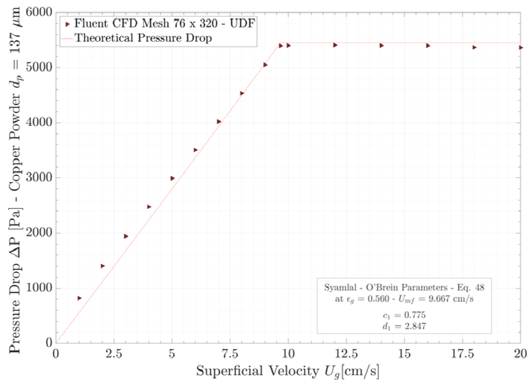
Figure 8. Pressure drop through the bed as function of the superficial gas velocity: comparison between theoretical pressure drop (red dashed line) and CFD calculation (black triangle). CFD calculations were obtained by implementing the parametric model of Syamlal-O'Brien: parameters of this model are shown in the table.
