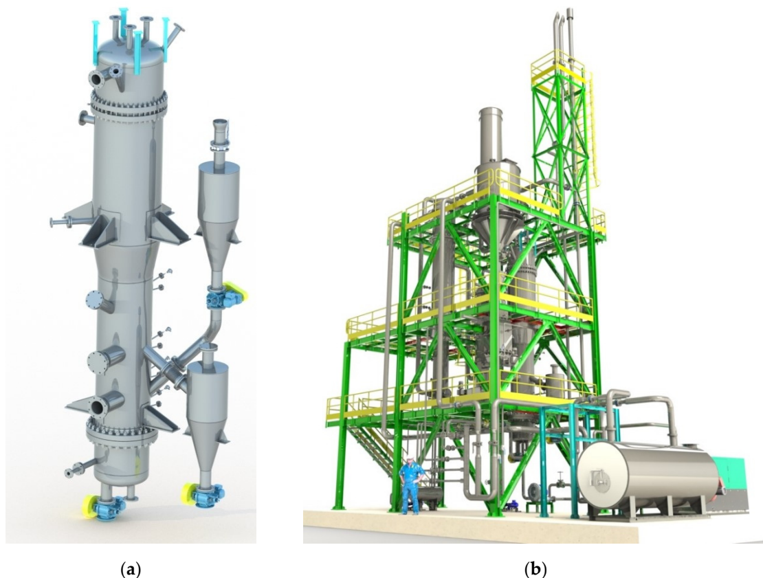
Figure 1. ENEA's 1 MW th Internally Circulating Bubbling Fluidized Bed (ICBFB) pilot plant: (a) Gasifier details; (b) Whole pilot plant layout: it is visible the biomass feeding system, the gasifier, the heat exchanger and the syngas cleaning system.
