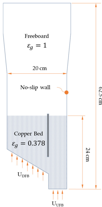
Figure 7. Schematic representation of the cold model used to investigate the hydrodynamic behavior of the ENEA's ICBFB reactor. In the table, characterizing properties of solid particles composing the inert bed material and fluidizing condition for the two chambers are collected.
