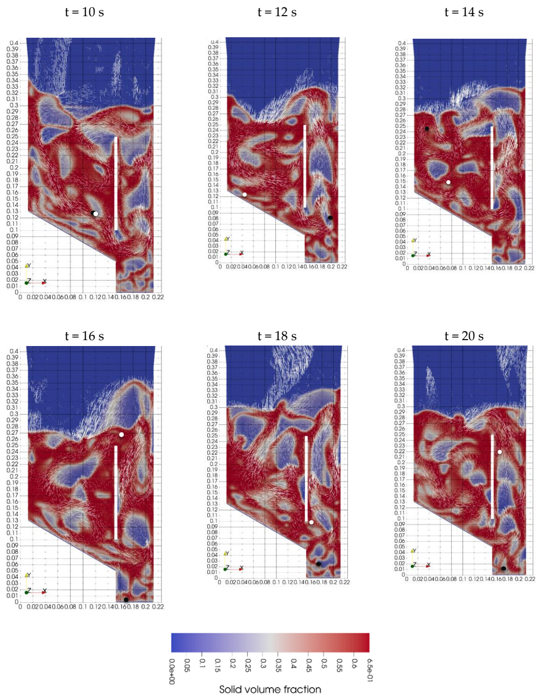
Figure 13. Visual representation of equivalent char particles position inside cold model reactor at different simulation time: white dot for particle of diameter \bar{d}_p = 0.22\text{ mm} ; black dot for particle of diameter \bar{d}_p = 0.27\text{ mm} . Images also show the instantaneous granular solid phase volume fraction and the solid velocity field.
