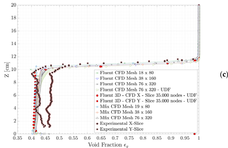
Figure 6. Averaged void fraction profiles as function of column diameter at (a) 4 cm and (b) 8 cm above flow distribution plate; (c) function of column height (calculated as mean values of all grids at the same height). Comparison between experimental and numerical data averaged between 5 s and 40 s.
