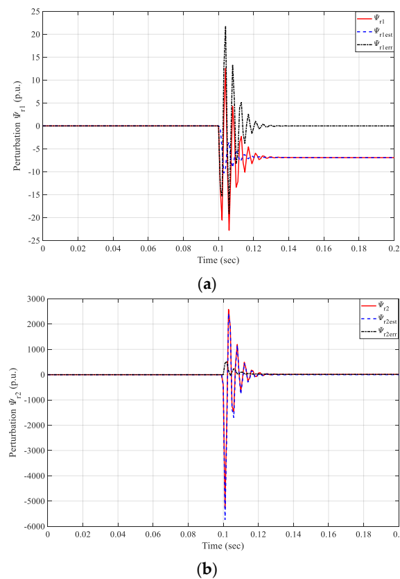
Figure 11. Disturbance rejection performance obtained under 20% voltage drop of rectifier. (a) Perturbation \Psi_{r1} and (b) perturbation \Psi_{r2} .
