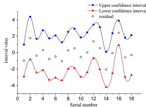
Figure 6. Residual confidence interval.
