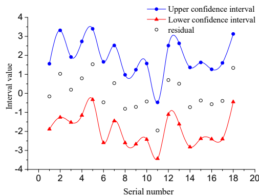
Figure 4. Residual confidence interval.
