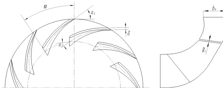
Figure 1. Main structural parameters of the guide vane.
