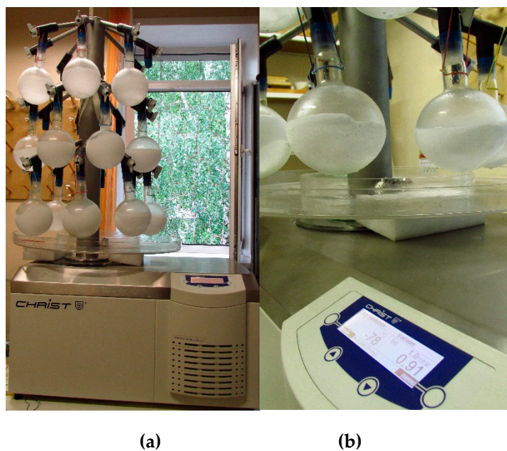
Figure S2: Equipment for freeze-drying of substance KS-6469: (a) General view); (b) The beginning of sublimation (a crust of ice is formed on the surface of the flask).
