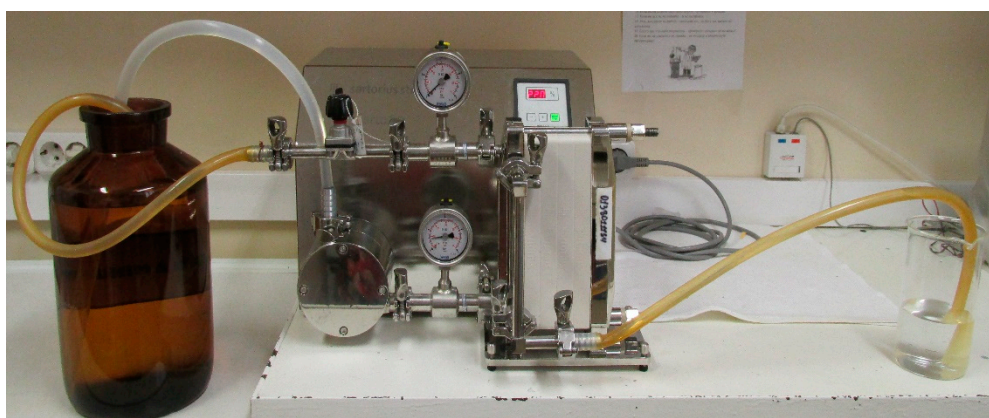
Figure S5: Equipment for tangential filtration of the substance solution KS-6469 (general view)
