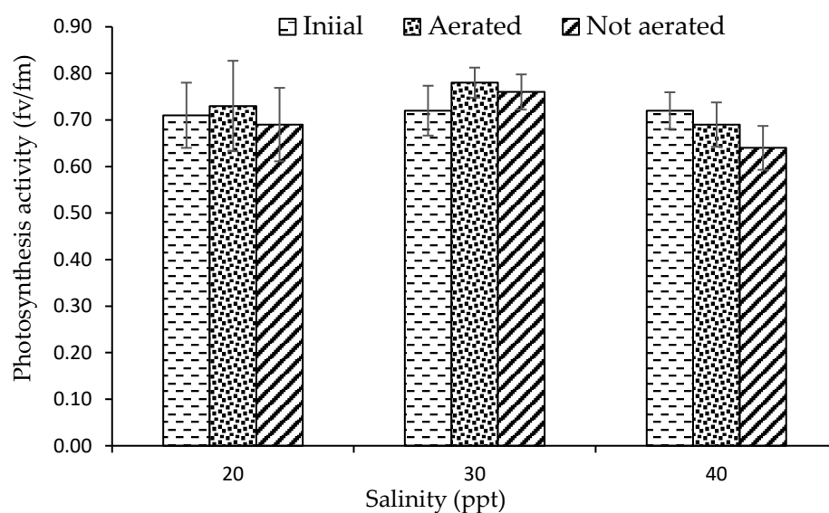
Figure. S1 Photosynthesis efficiency (fv / fm) at three salinity levels at initial (0 h) and final (24 h) nutrient uptake with and without aeration, with 30 g/L Caulerpa lentillifera density. The error bars indicate standard deviation. n=3
